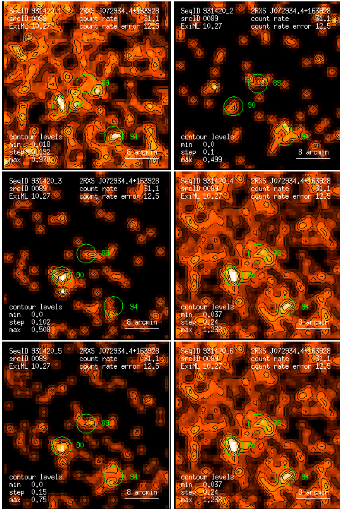
Figure 89: RASS 931420: detection 0089: band rate images, Gaussian filter: (1) PSPC channels 11 – 41, (2) 52 – 90, (3) 91 – 201, (4) 11 – 235, (5) 52 – 201, (6) 11 – 201. Broad band rates in counts/ks. Band rate contour levels in counts/ks/arcmin 2 .
