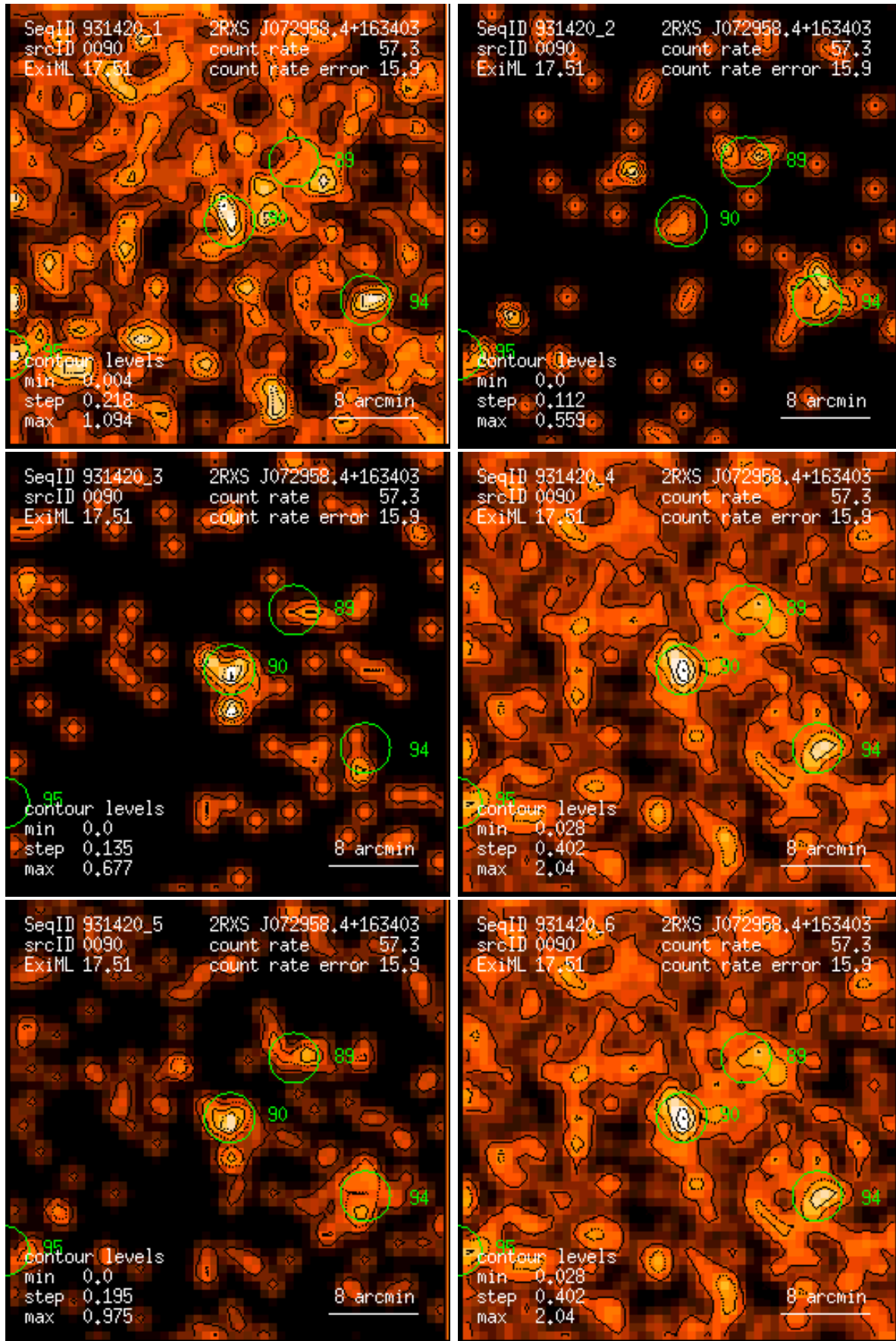
Figure 90: RASS 931420: detection 0090: band rate images, Gaussian filter: (1) PSPC channels 11 – 41, (2) 52 – 90, (3) 91 – 201, (4) 11 – 235, (5) 52 – 201, (6) 11 – 201. Broad band rates in counts/ks. Band rate contour levels in counts/ks/arcmin 2 .
