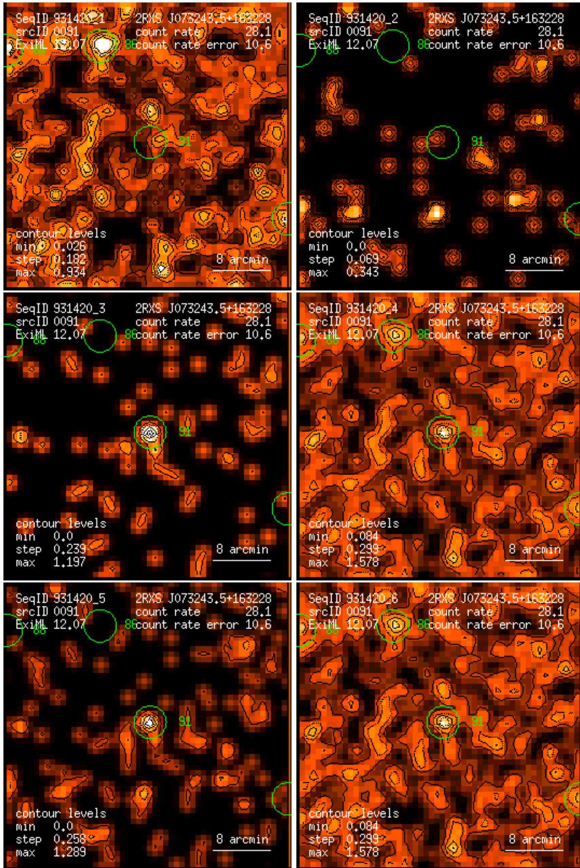
Figure 91: RASS 931420: detection 0091: band rate images, Gaussian filter: (1) PSPC channels 11 – 41, (2) 52 – 90, (3) 91 – 201, (4) 11 – 235, (5) 52 – 201, (6) 11 – 201. Broad band rates in counts/ks. Band rate contour levels in counts/ks/arcmin 2 .
