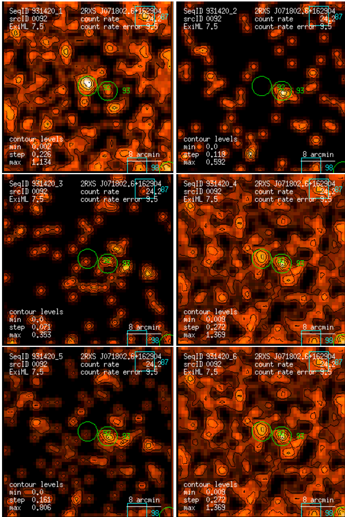
Figure 92: RASS 931420: detection 0092: band rate images, Gaussian filter: (1) PSPC channels 11 – 41, (2) 52 – 90, (3) 91 – 201, (4) 11 – 235, (5) 52 – 201, (6) 11 – 201. Broad band rates in counts/ks. Band rate contour levels in counts/ks/arcmin 2 .
