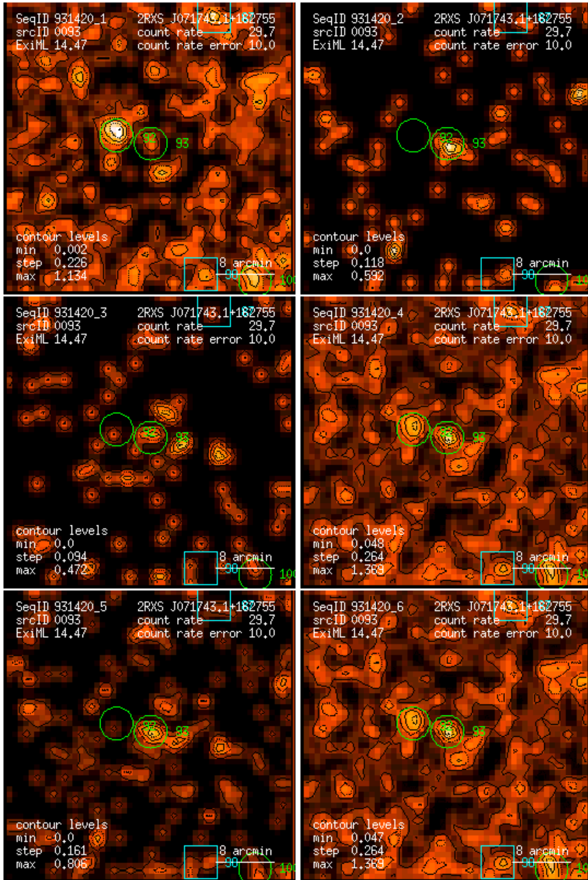
Figure 93: RASS 931420: detection 0093: band rate images, Gaussian filter: (1) PSPC channels 11 – 41, (2) 52 – 90, (3) 91 – 201, (4) 11 – 235, (5) 52 – 201, (6) 11 – 201. Broad band rates in counts/ks. Band rate contour levels in counts/ks/arcmin 2 .
