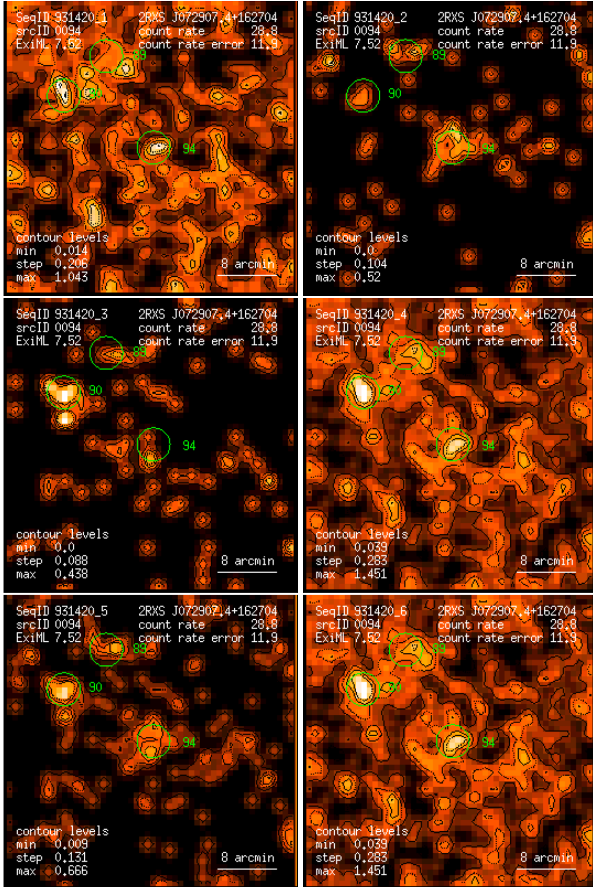
Figure 94: RASS 931420: detection 0094: band rate images, Gaussian filter: (1) PSPC channels 11 – 41, (2) 52 – 90, (3) 91 – 201, (4) 11 – 235, (5) 52 – 201, (6) 11 – 201. Broad band rates in counts/ks. Band rate contour levels in counts/ks/arcmin 2 .
