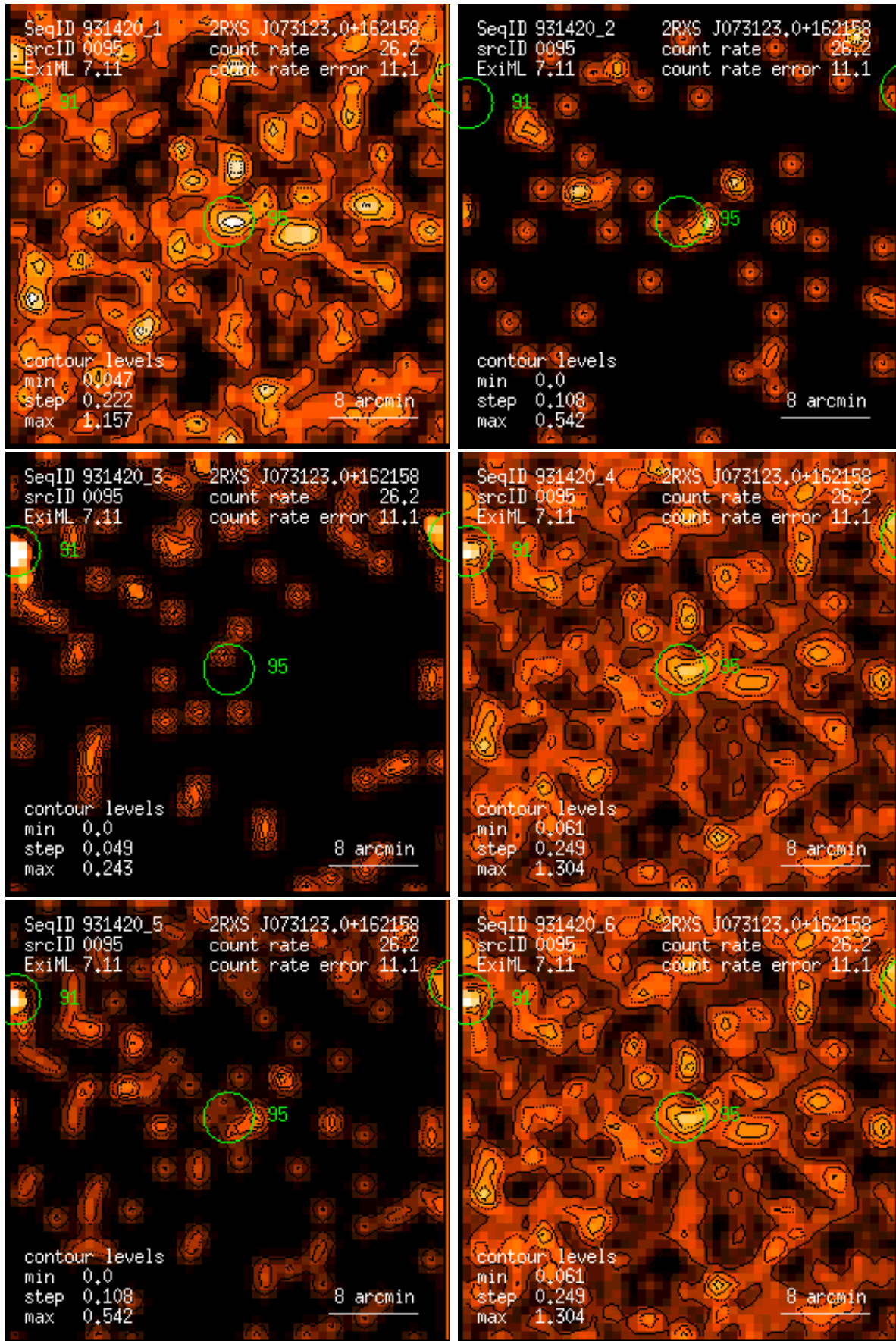
Figure 95: RASS 931420: detection 0095: band rate images, Gaussian filter: (1) PSPC channels 11 – 41, (2) 52 – 90, (3) 91 – 201, (4) 11 – 235, (5) 52 – 201, (6) 11 – 201. Broad band rates in counts/ks. Band rate contour levels in counts/ks/arcmin 2 .
