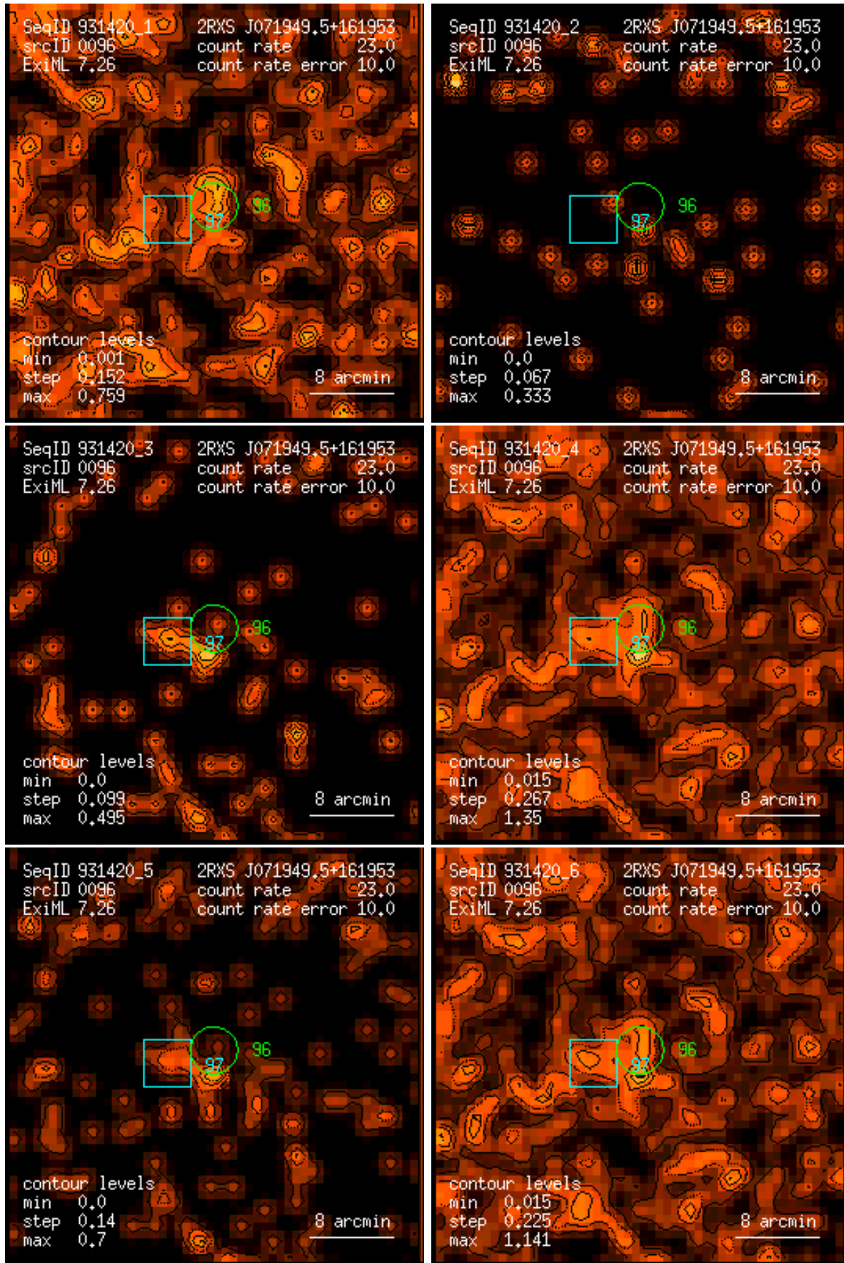
Figure 96: RASS 931420: detection 0096: band rate images, Gaussian filter: (1) PSPC channels 11 – 41, (2) 52 – 90, (3) 91 – 201, (4) 11 – 235, (5) 52 – 201, (6) 11 – 201. Broad band rates in counts/ks. Band rate contour levels in counts/ks/arcmin 2 .
