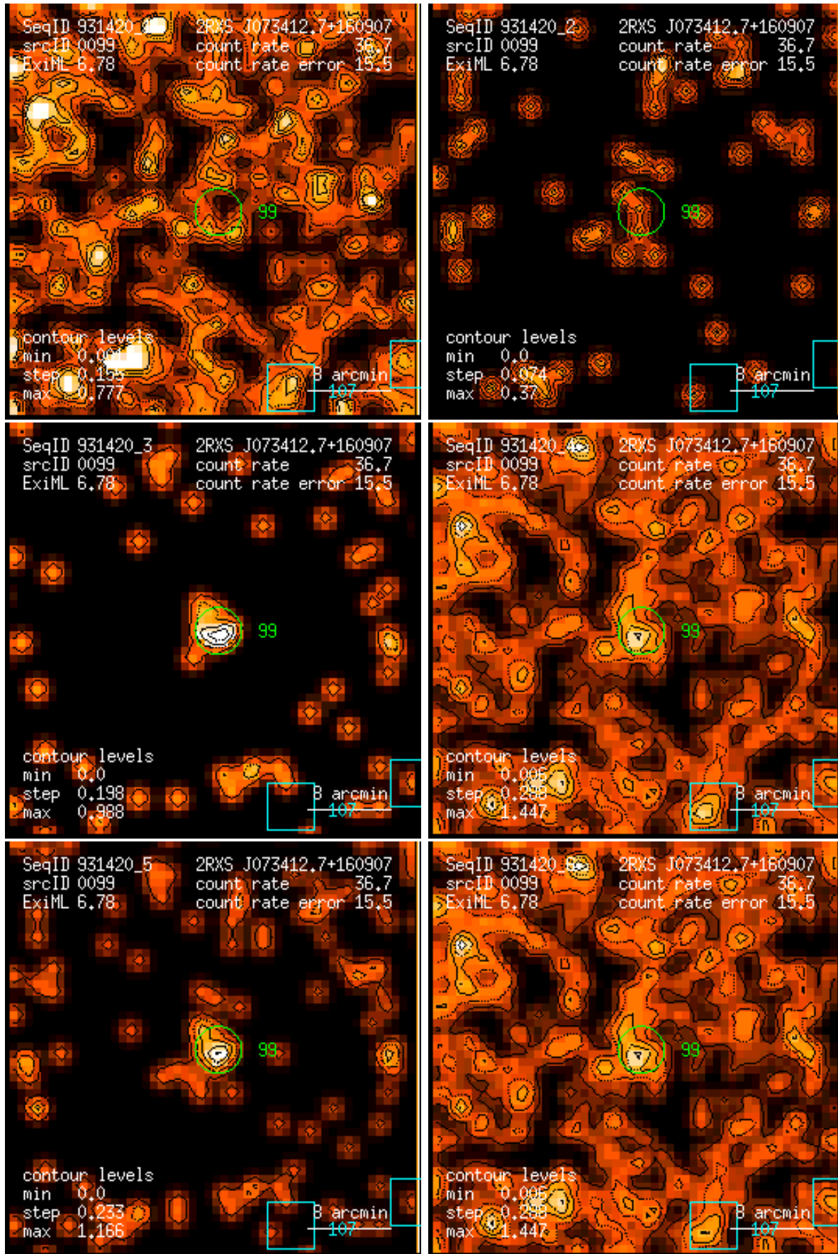
Figure 99: RASS 931420: detection 0099: band rate images, Gaussian filter: (1) PSPC channels 11 – 41, (2) 52 – 90, (3) 91 – 201, (4) 11 – 235, (5) 52 – 201, (6) 11 – 201. Broad band rates in counts/ks. Band rate contour levels in counts/ks/arcmin 2 .
