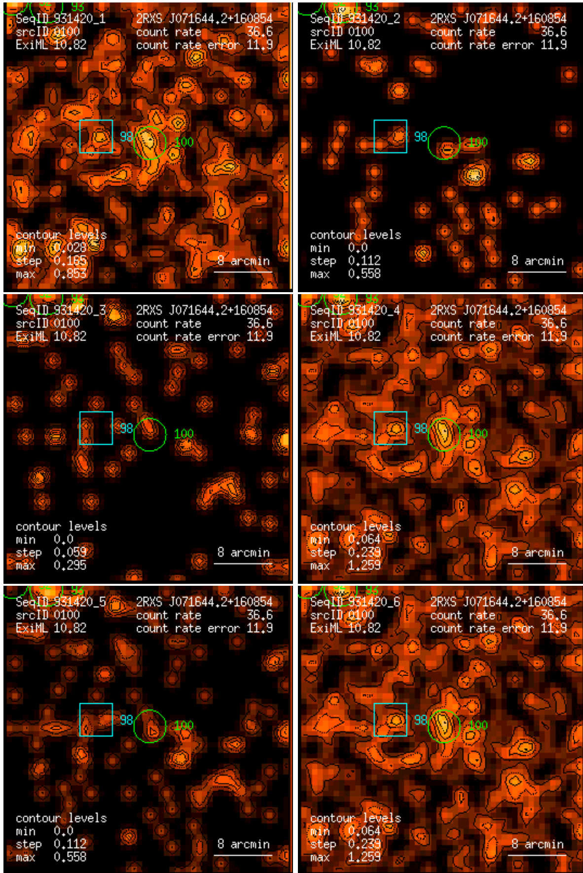
Figure 100: RASS 931420: detection 0100: band rate images, Gaussian filter: (1) PSPC channels 11 – 41, (2) 52 – 90, (3) 91 – 201, (4) 11 – 235, (5) 52 – 201, (6) 11 – 201. Broad band rates in counts/ks. Band rate contour levels in counts/ks/arcmin 2 .
