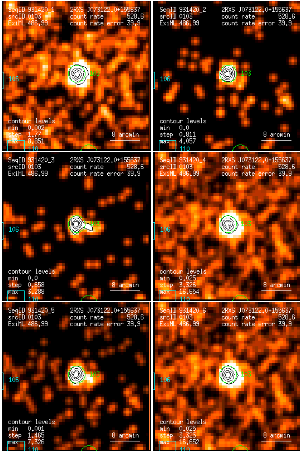
Figure 103: RASS 931420: detection 0103: band rate images, Gaussian filter: (1) PSPC channels 11 – 41, (2) 52 – 90, (3) 91 – 201, (4) 11 – 235, (5) 52 – 201, (6) 11 – 201. Broad band rates in counts/ks. Band rate contour levels in counts/ks/arcmin 2 .
