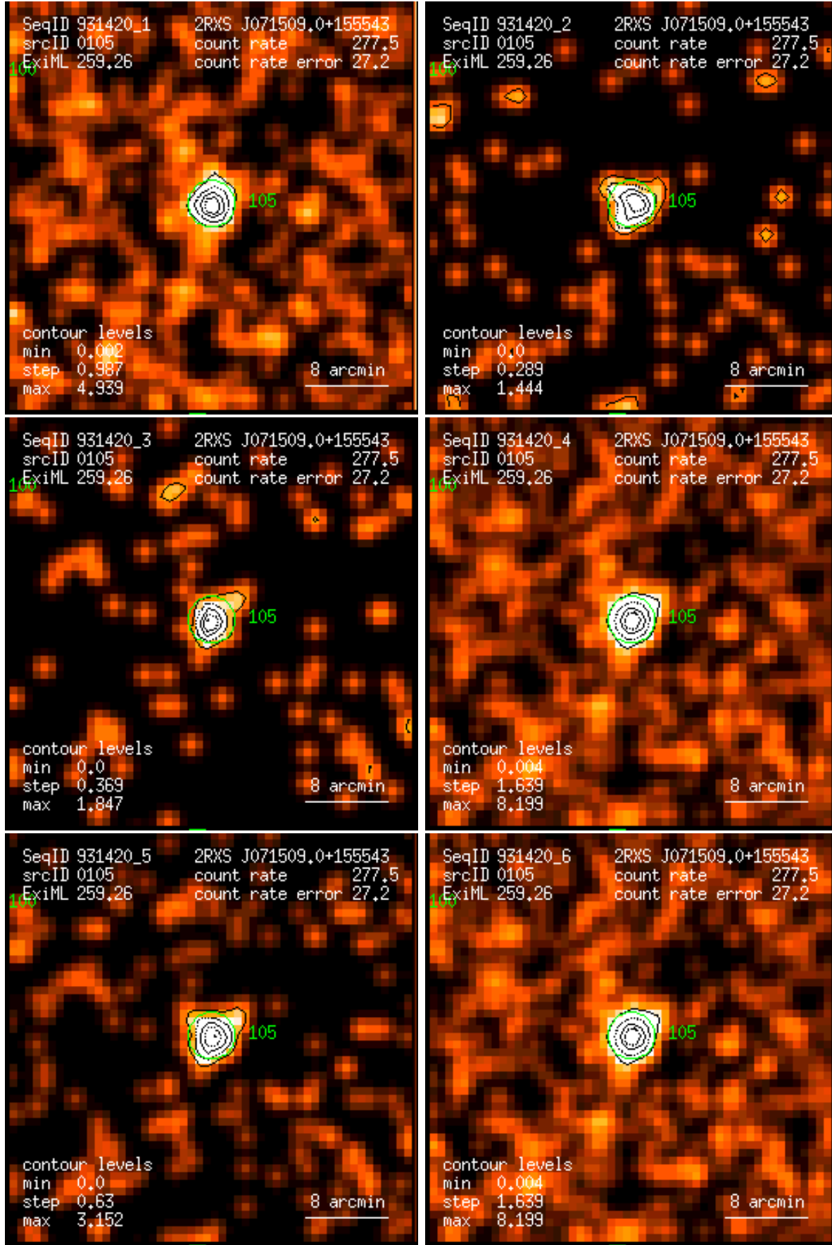
Figure 105: RASS 931420: detection 0105: band rate images, Gaussian filter: (1) PSPC channels 11 – 41, (2) 52 – 90, (3) 91 – 201, (4) 11 – 235, (5) 52 – 201, (6) 11 – 201. Broad band rates in counts/ks. Band rate contour levels in counts/ks/arcmin 2 .
