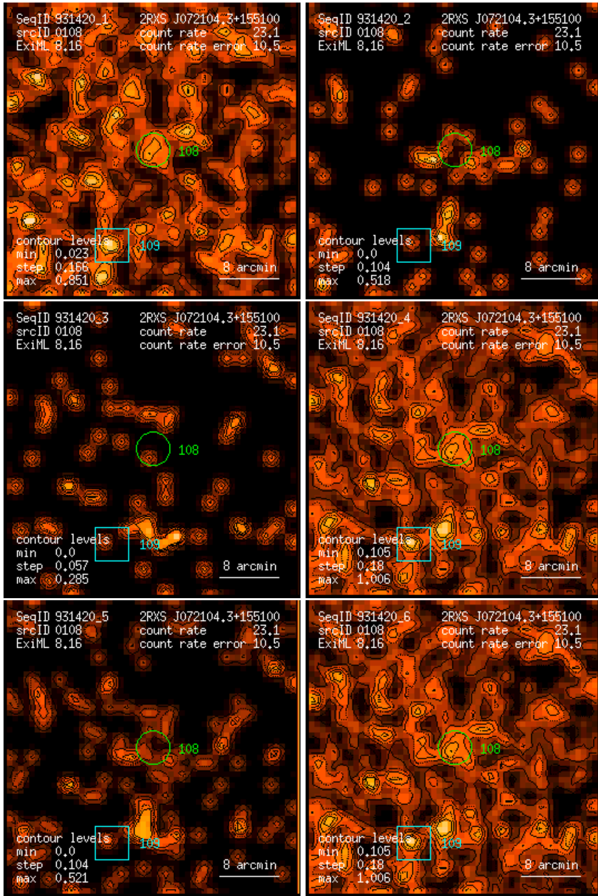
Figure 108: RASS 931420: detection 0108: band rate images, Gaussian filter: (1) PSPC channels 11 – 41, (2) 52 – 90, (3) 91 – 201, (4) 11 – 235, (5) 52 – 201, (6) 11 – 201. Broad band rates in counts/ks. Band rate contour levels in counts/ks/arcmin 2 .
