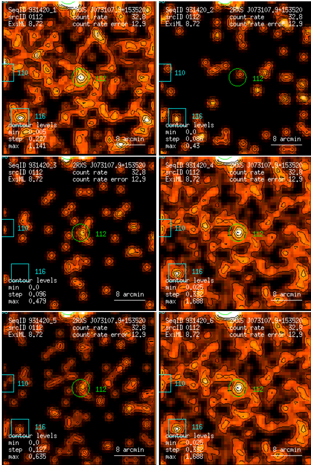
Figure 112: RASS 931420: detection 0112: band rate images, Gaussian filter: (1) PSPC channels 11 – 41, (2) 52 – 90, (3) 91 – 201, (4) 11 – 235, (5) 52 – 201, (6) 11 – 201. Broad band rates in counts/ks. Band rate contour levels in counts/ks/arcmin 2 .
