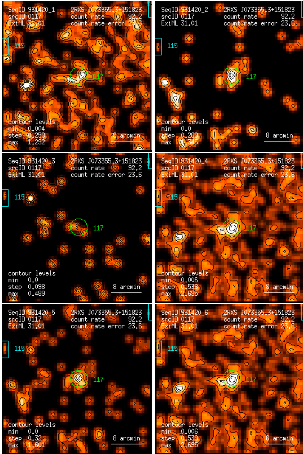
Figure 117: RASS 931420: detection 0117: band rate images, Gaussian filter: (1) PSPC channels 11 – 41, (2) 52 – 90, (3) 91 – 201, (4) 11 – 235, (5) 52 – 201, (6) 11 – 201. Broad band rates in counts/ks. Band rate contour levels in counts/ks/arcmin 2 .
