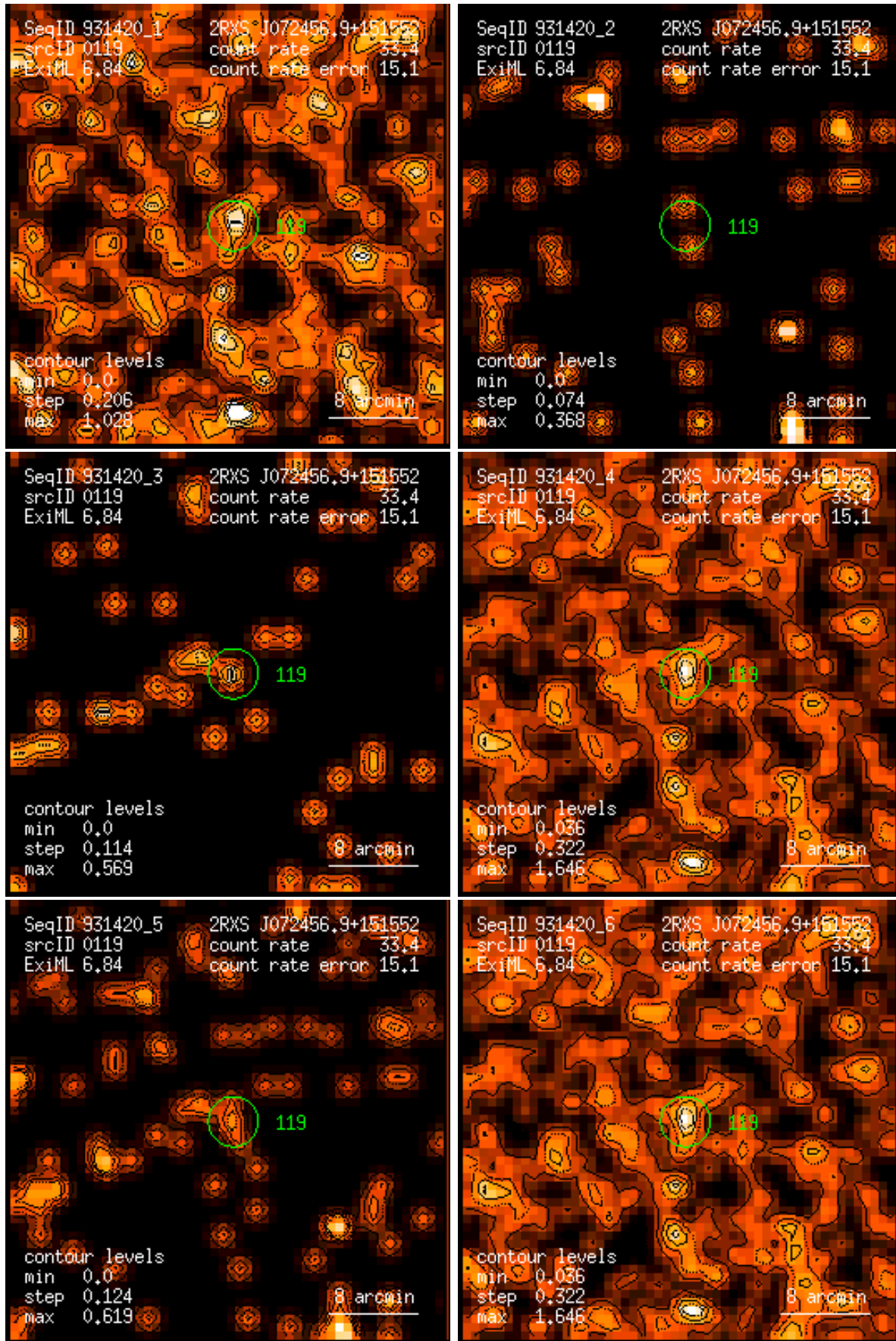
Figure 119: RASS 931420: detection 0119: band rate images, Gaussian filter: (1) PSPC channels 11 – 41, (2) 52 – 90, (3) 91 – 201, (4) 11 – 235, (5) 52 – 201, (6) 11 – 201. Broad band rates in counts/ks. Band rate contour levels in counts/ks/arcmin 2 .
