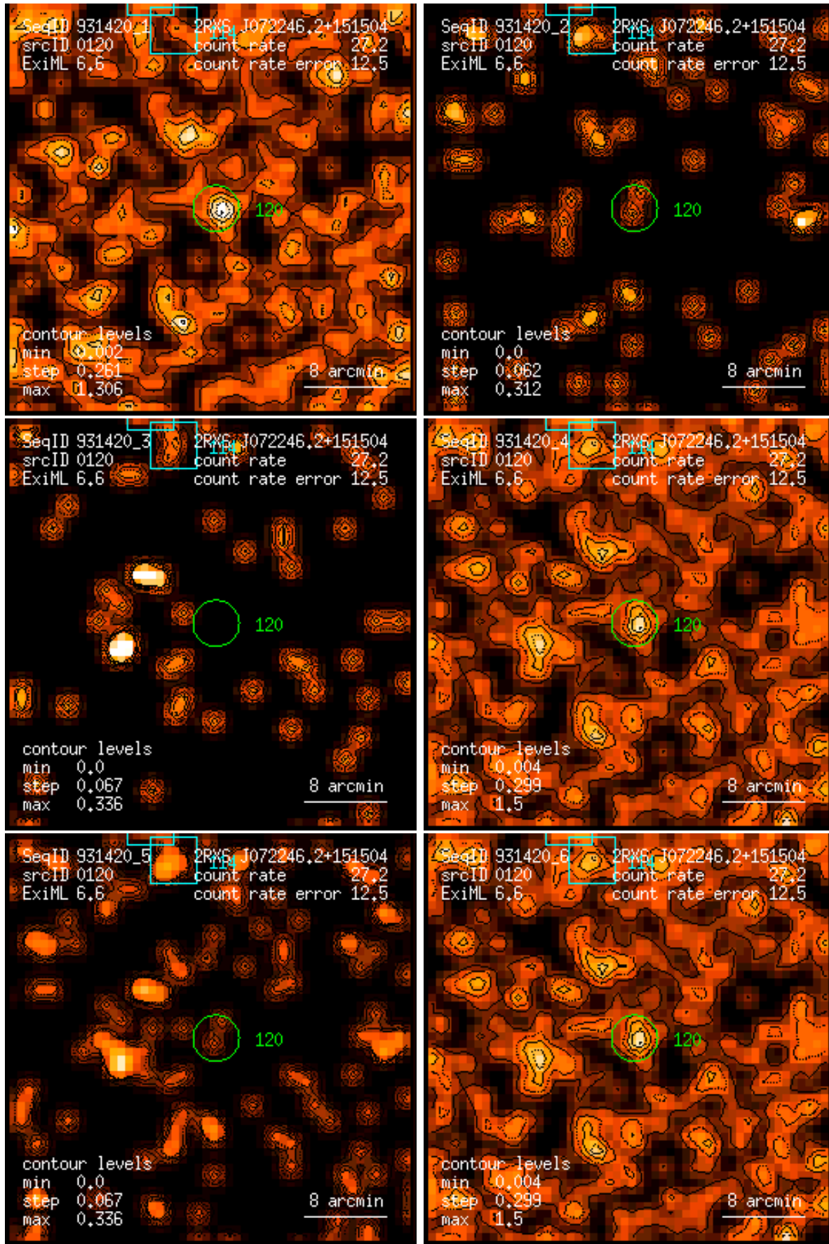
Figure 120: RASS 931420: detection 0120: band rate images, Gaussian filter: (1) PSPC channels 11 – 41, (2) 52 – 90, (3) 91 – 201, (4) 11 – 235, (5) 52 – 201, (6) 11 – 201. Broad band rates in counts/ks. Band rate contour levels in counts/ks/arcmin 2 .
