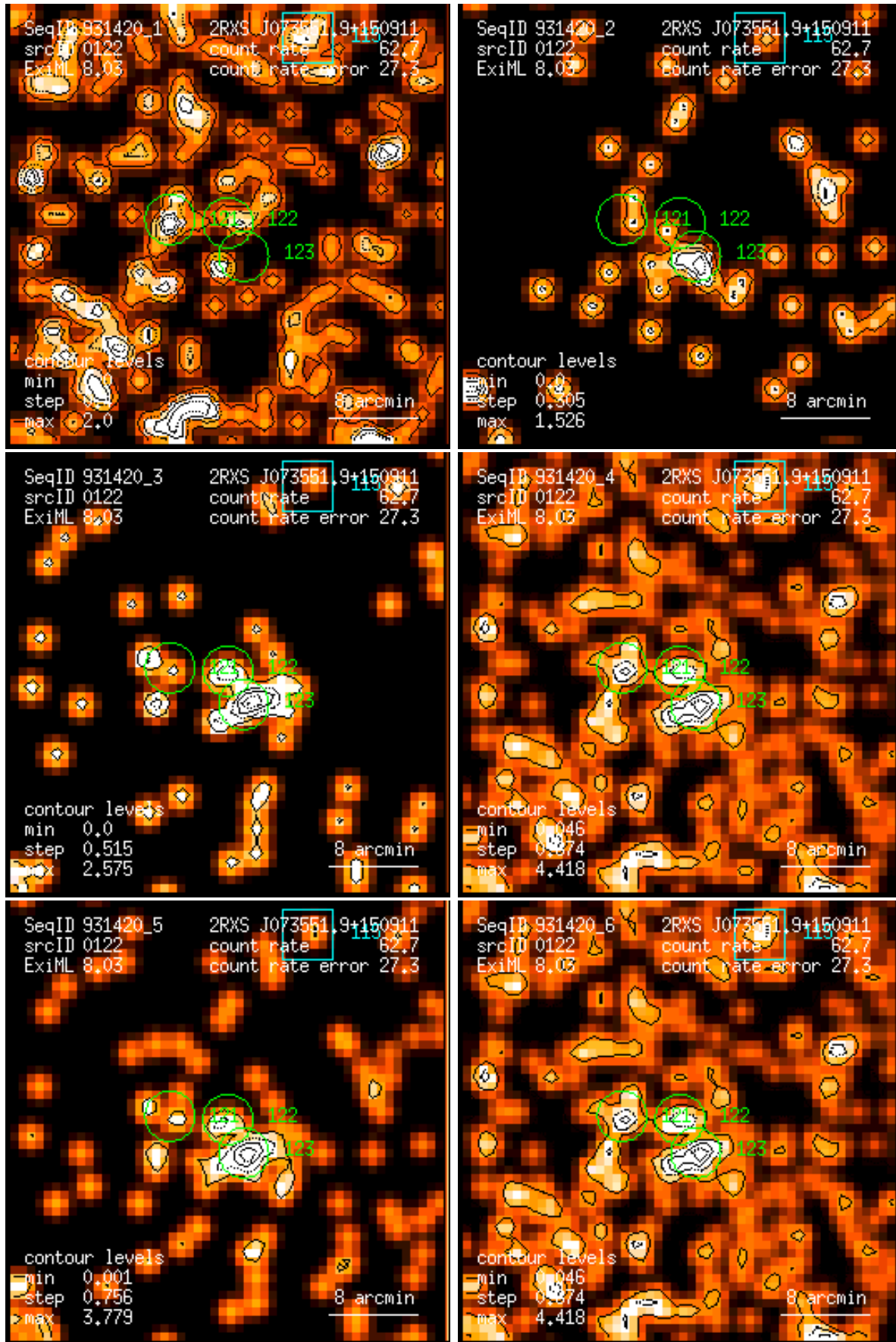
Figure 122: RASS 931420: detection 0122: band rate images, Gaussian filter: (1) PSPC channels 11 – 41, (2) 52 – 90, (3) 91 – 201, (4) 11 – 235, (5) 52 – 201, (6) 11 – 201. Broad band rates in counts/ks. Band rate contour levels in counts/ks/arcmin 2 .
