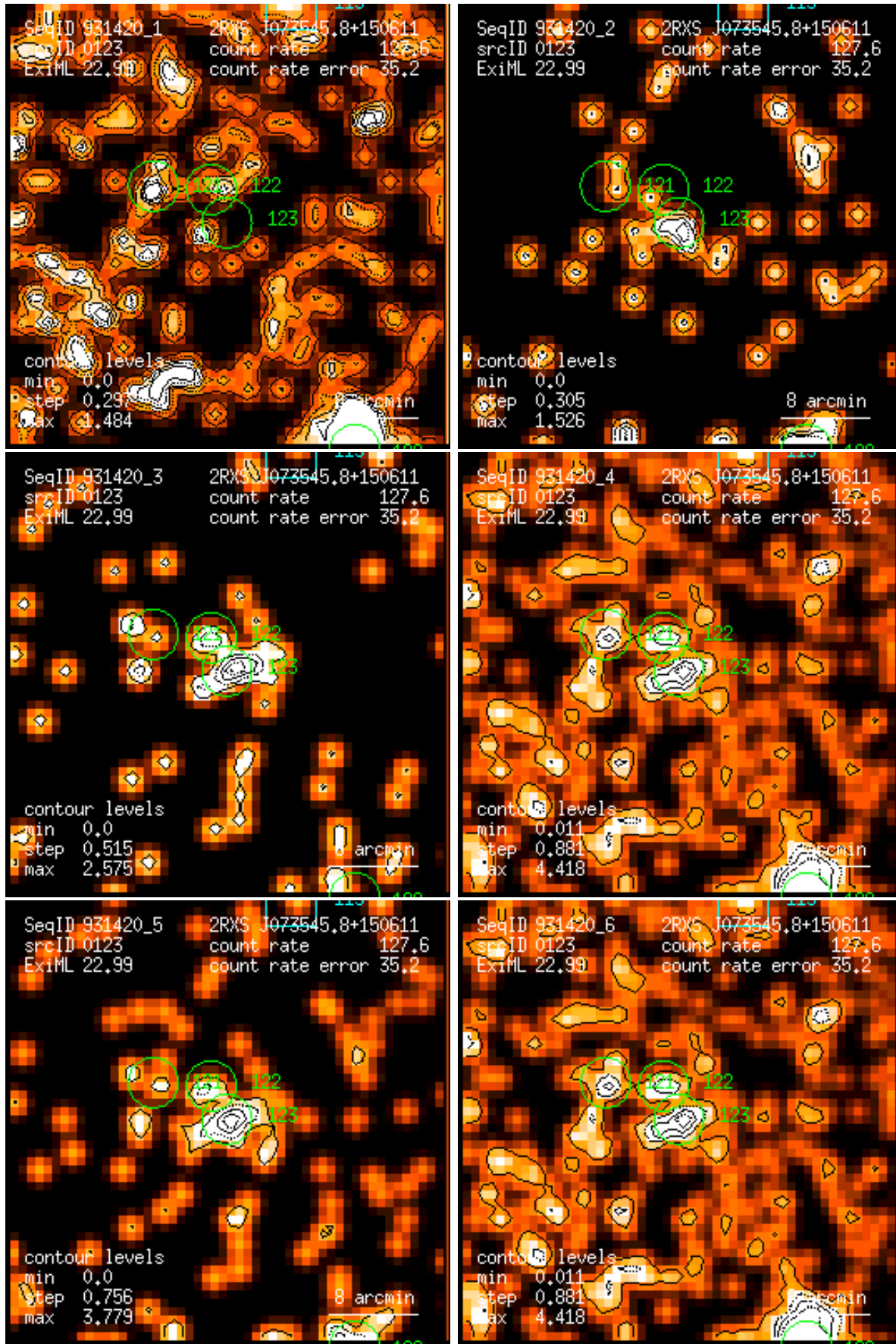
Figure 123: RASS 931420: detection 0123: band rate images, Gaussian filter: (1) PSPC channels 11 – 41, (2) 52 – 90, (3) 91 – 201, (4) 11 – 235, (5) 52 – 201, (6) 11 – 201. Broad band rates in counts/ks. Band rate contour levels in counts/ks/arcmin 2 .
