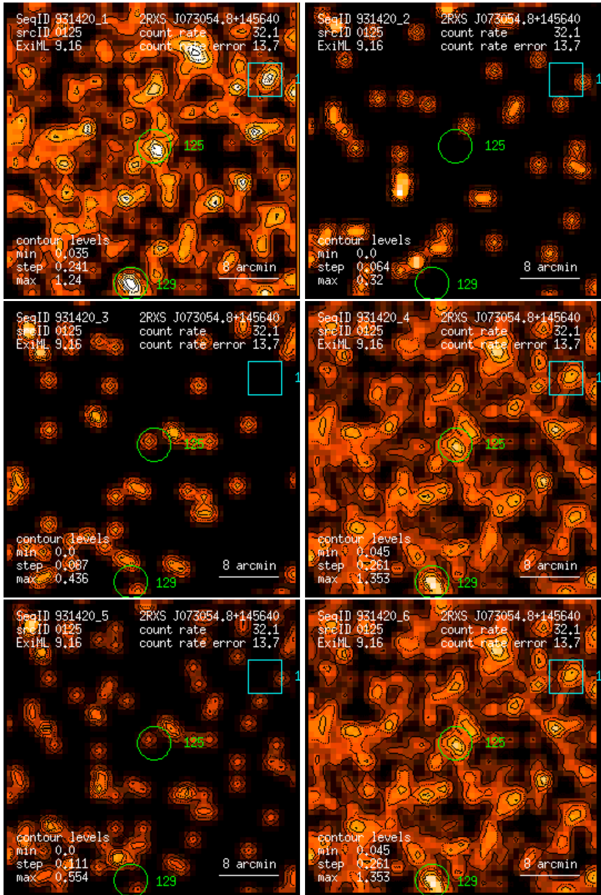
Figure 125: RASS 931420: detection 0125: band rate images, Gaussian filter: (1) PSPC channels 11 – 41, (2) 52 – 90, (3) 91 – 201, (4) 11 – 235, (5) 52 – 201, (6) 11 – 201. Broad band rates in counts/ks. Band rate contour levels in counts/ks/arcmin 2 .
