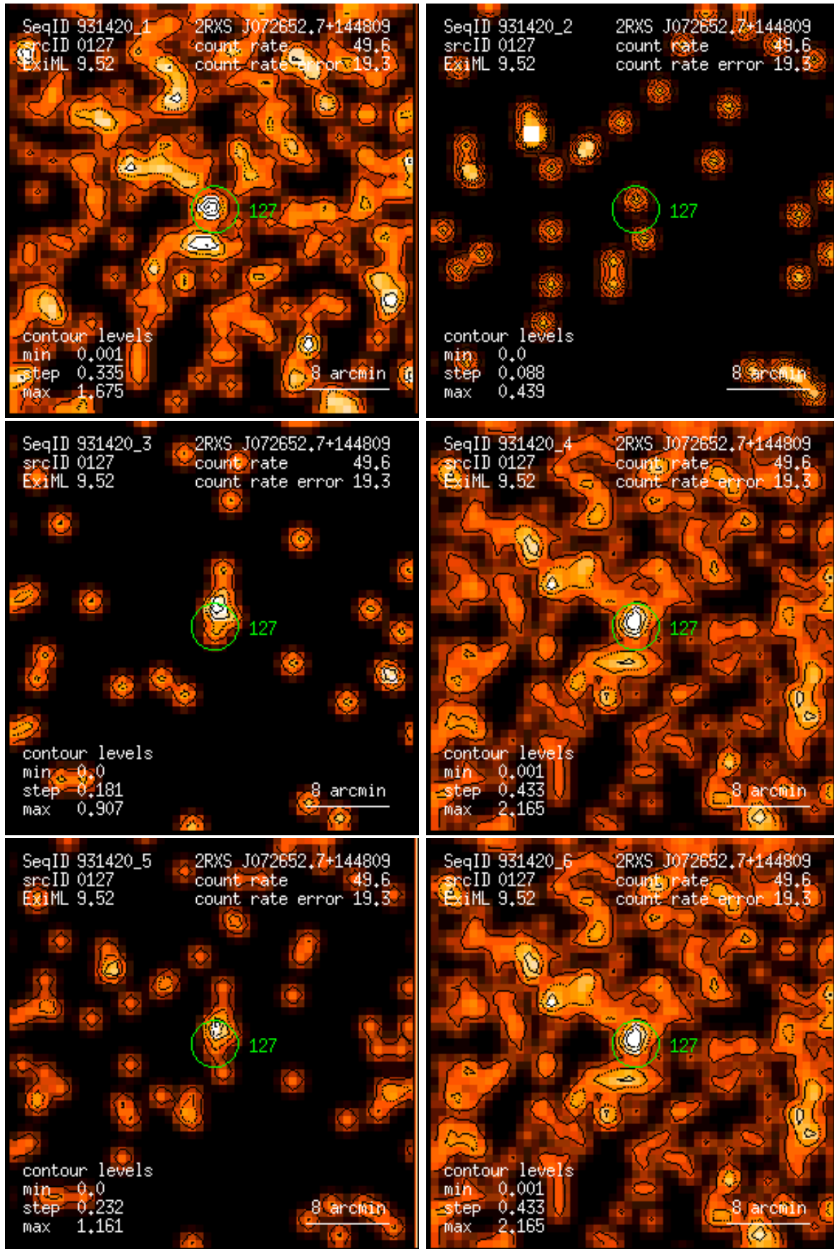
Figure 127: RASS 931420: detection 0127: band rate images, Gaussian filter: (1) PSPC channels 11 – 41, (2) 52 – 90, (3) 91 – 201, (4) 11 – 235, (5) 52 – 201, (6) 11 – 201. Broad band rates in counts/ks. Band rate contour levels in counts/ks/arcmin 2 .
