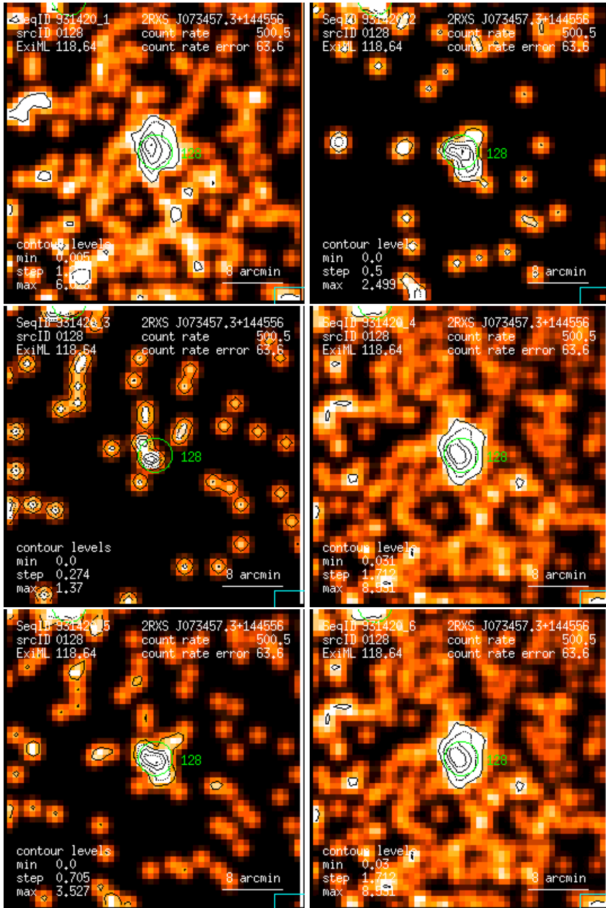
Figure 128: RASS 931420: detection 0128: band rate images, Gaussian filter: (1) PSPC channels 11 – 41, (2) 52 – 90, (3) 91 – 201, (4) 11 – 235, (5) 52 – 201, (6) 11 – 201. Broad band rates in counts/ks. Band rate contour levels in counts/ks/arcmin 2 .
