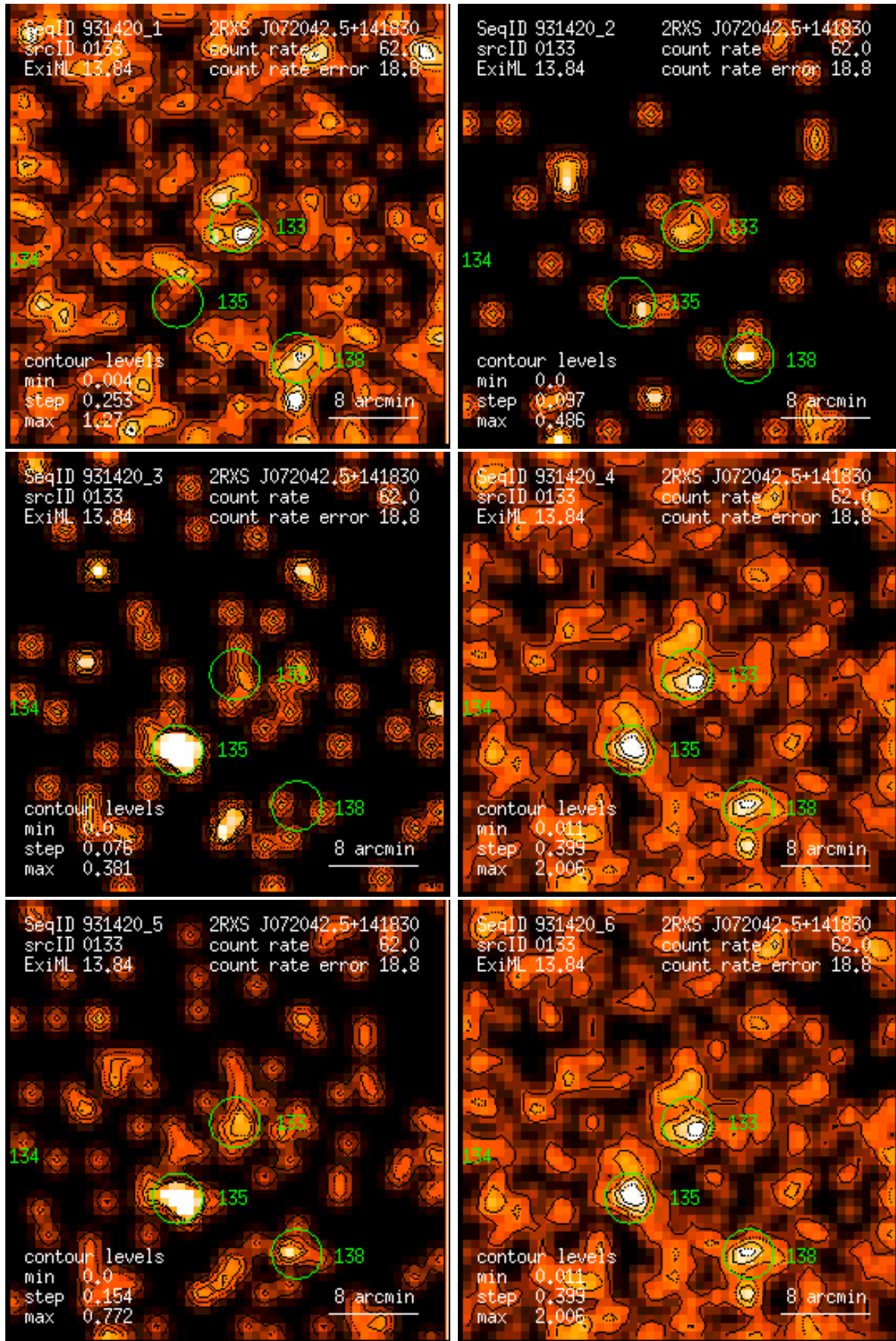
Figure 133: RASS 931420: detection 0133: band rate images, Gaussian filter: (1) PSPC channels 11 – 41, (2) 52 – 90, (3) 91 – 201, (4) 11 – 235, (5) 52 – 201, (6) 11 – 201. Broad band rates in counts/ks. Band rate contour levels in counts/ks/arcmin 2 .
