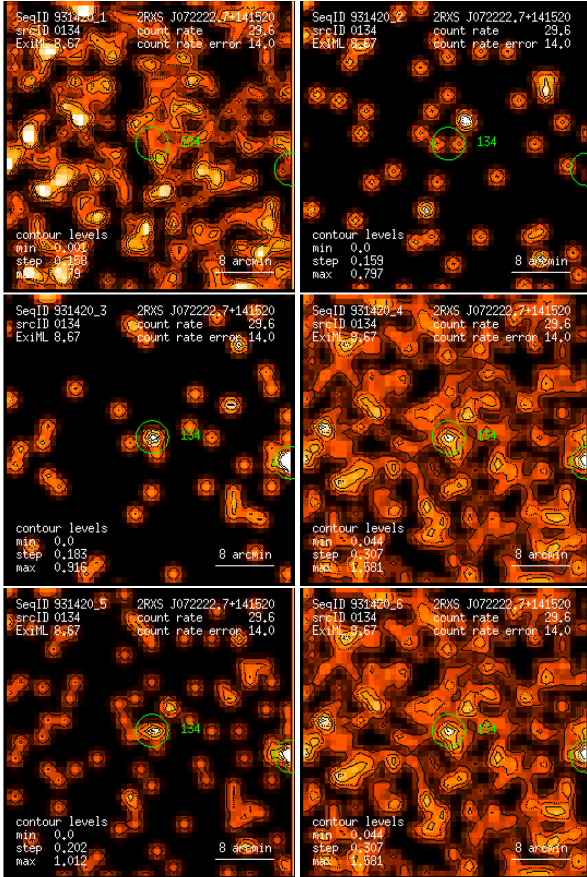
Figure 134: RASS 931420: detection 0134: band rate images, Gaussian filter: (1) PSPC channels 11 – 41, (2) 52 – 90, (3) 91 – 201, (4) 11 – 235, (5) 52 – 201, (6) 11 – 201. Broad band rates in counts/ks. Band rate contour levels in counts/ks/arcmin 2 .
