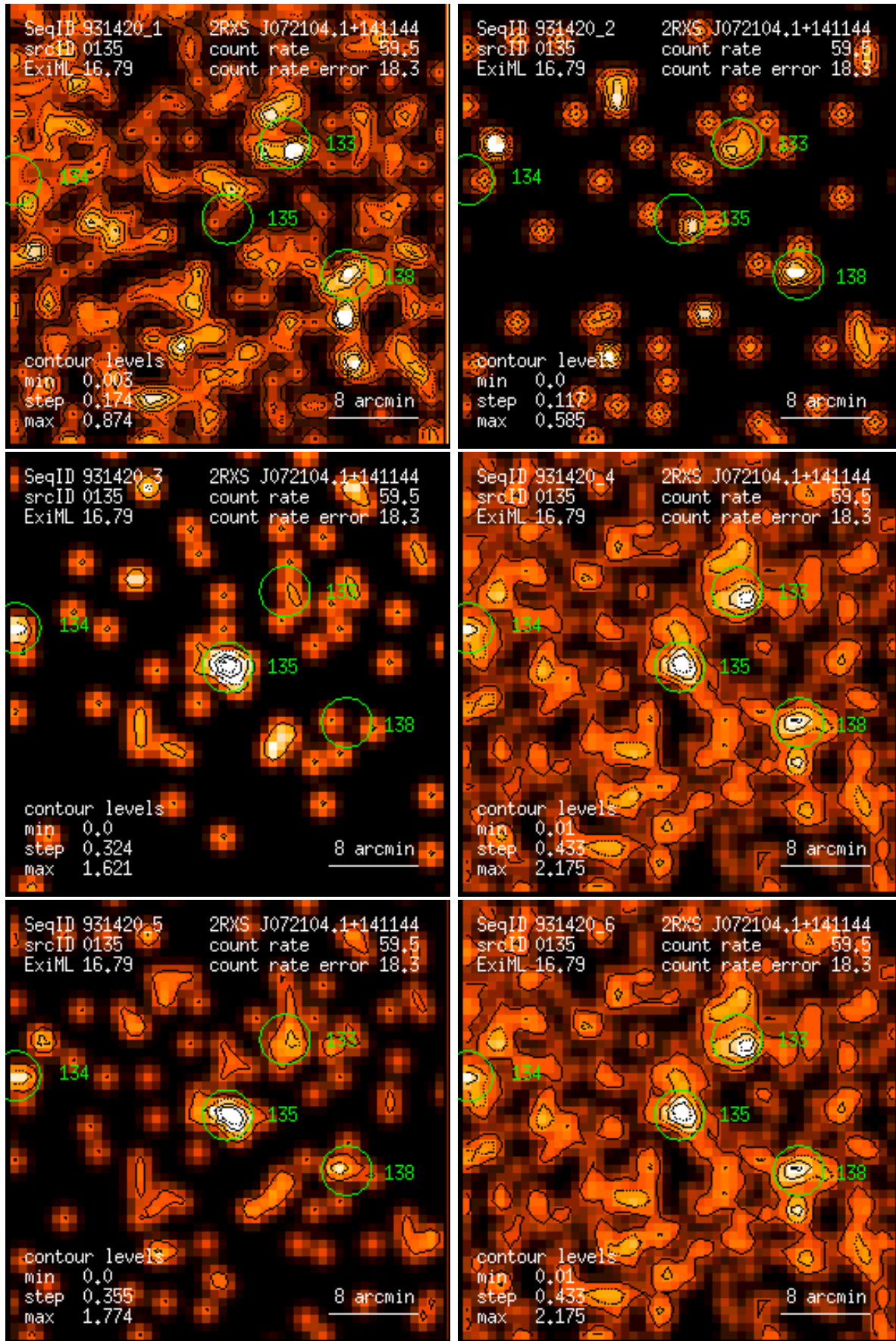
Figure 135: RASS 931420: detection 0135: band rate images, Gaussian filter: (1) PSPC channels 11 – 41, (2) 52 – 90, (3) 91 – 201, (4) 11 – 235, (5) 52 – 201, (6) 11 – 201. Broad band rates in counts/ks. Band rate contour levels in counts/ks/arcmin 2 .
