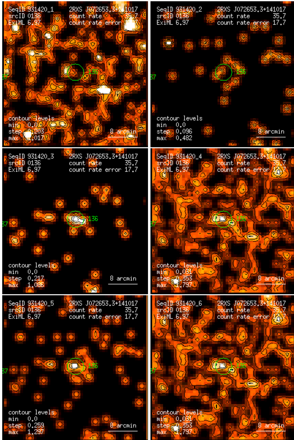
Figure 136: RASS 931420: detection 0136: band rate images, Gaussian filter: (1) PSPC channels 11 – 41, (2) 52 – 90, (3) 91 – 201, (4) 11 – 235, (5) 52 – 201, (6) 11 – 201. Broad band rates in counts/ks. Band rate contour levels in counts/ks/arcmin 2 .
