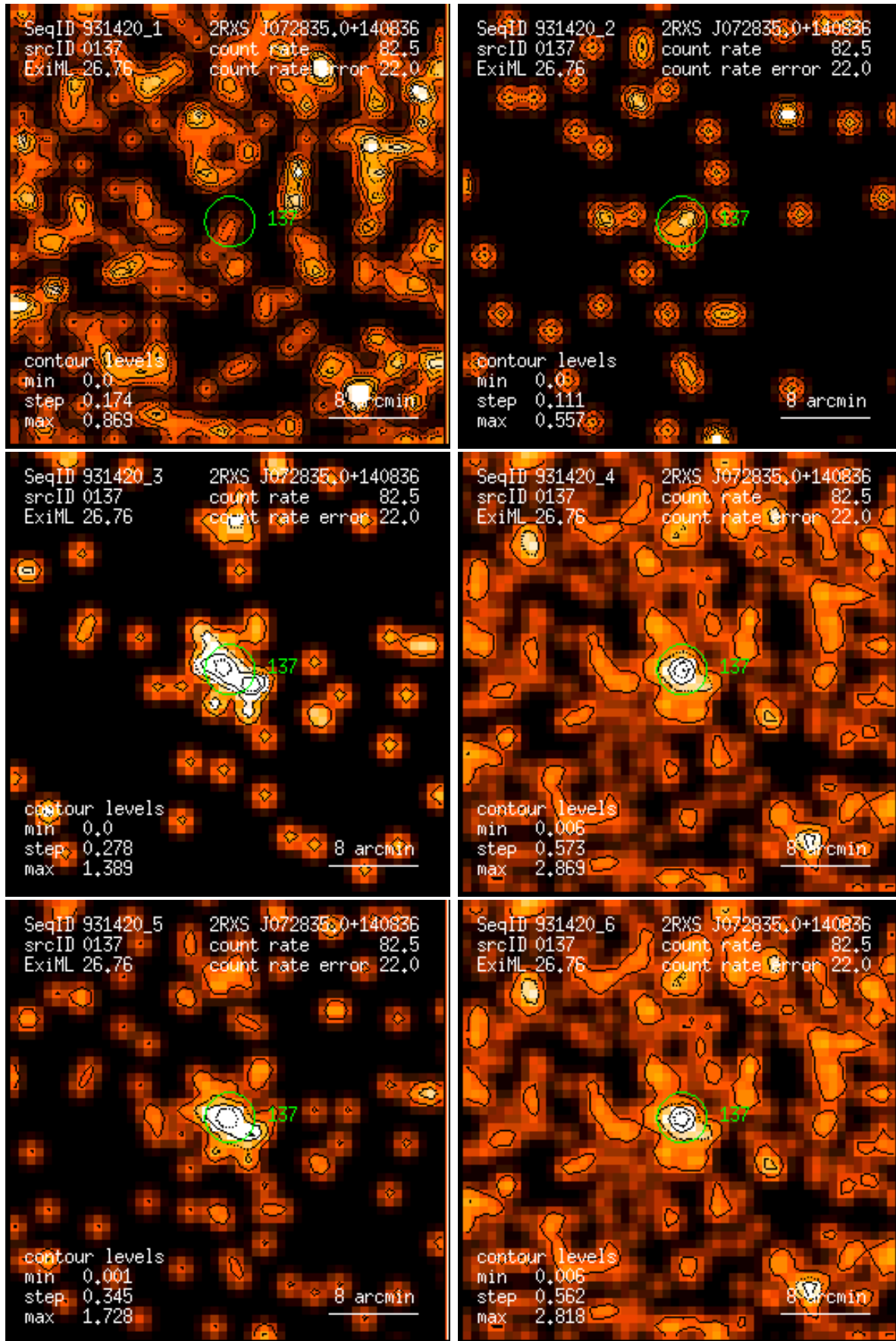
Figure 137: RASS 931420: detection 0137: band rate images, Gaussian filter: (1) PSPC channels 11 – 41, (2) 52 – 90, (3) 91 – 201, (4) 11 – 235, (5) 52 – 201, (6) 11 – 201. Broad band rates in counts/ks. Band rate contour levels in counts/ks/arcmin 2 .
