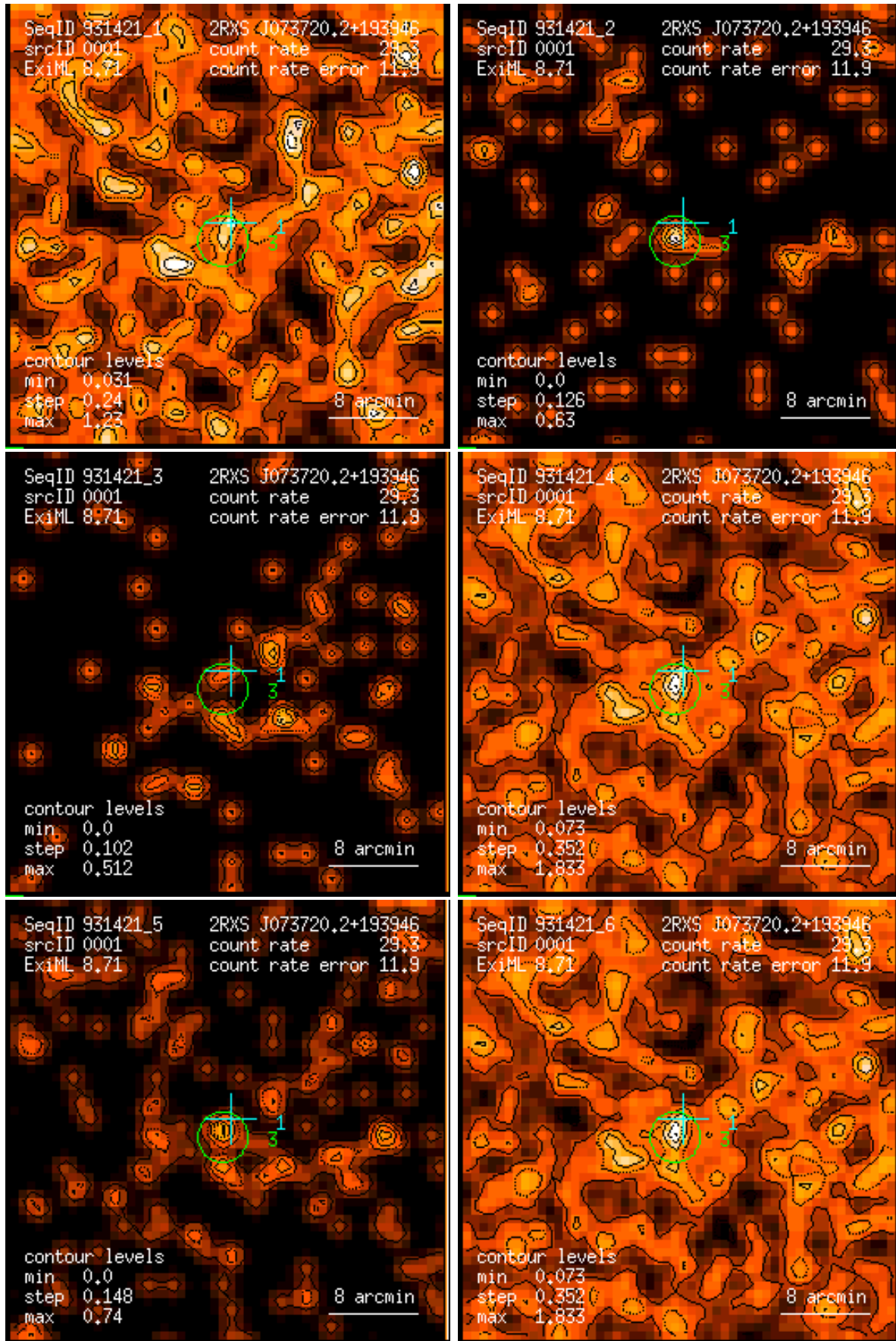
Figure 1: RASS 931421: detection 0001: band rate images, Gaussian filter: (1) PSPC channels 11 – 41, (2) 52 – 90, (3) 91 – 201, (4) 11 – 235, (5) 52 – 201, (6) 11 – 201. Broad band rates in counts/ks. Band rate contour levels in counts/ks/arcmin 2 .
