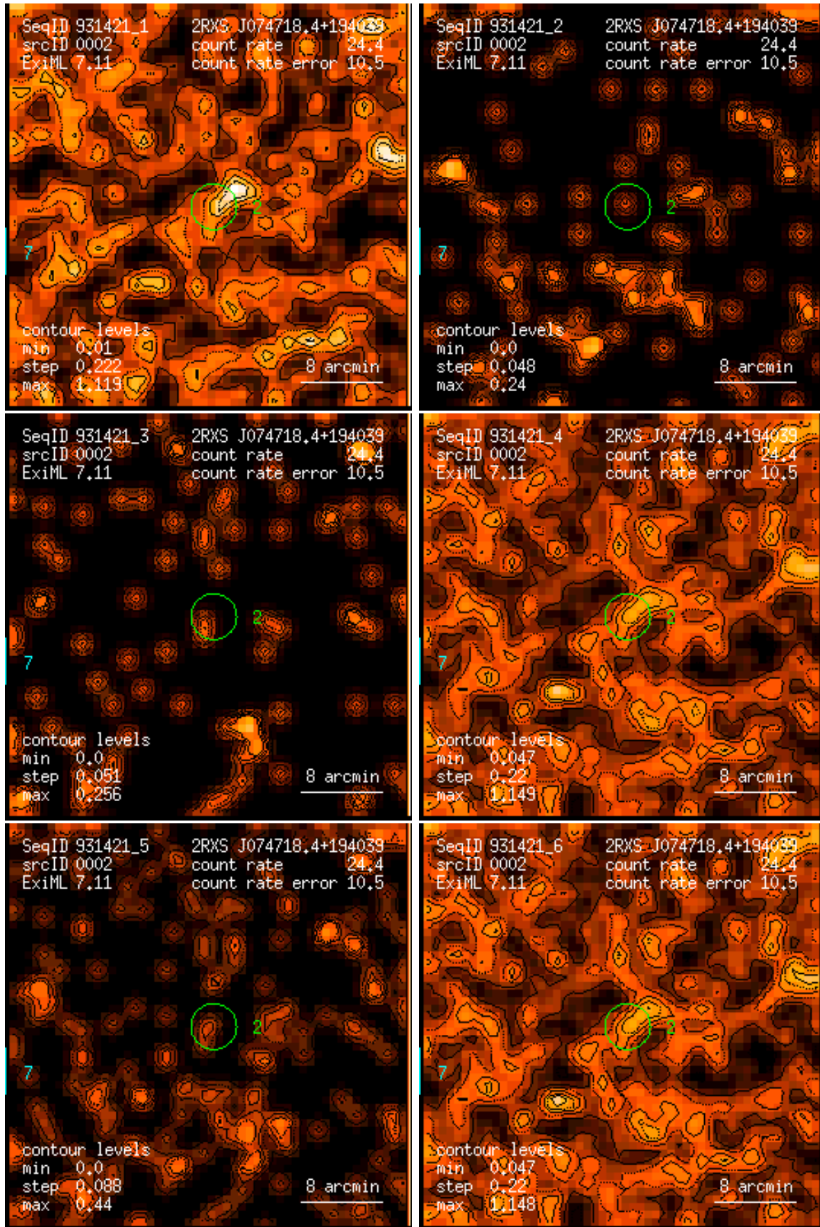
Figure 2: RASS 931421: detection 0002: band rate images, Gaussian filter: (1) PSPC channels 11 – 41, (2) 52 – 90, (3) 91 – 201, (4) 11 – 235, (5) 52 – 201, (6) 11 – 201. Broad band rates in counts/ks. Band rate contour levels in counts/ks/arcmin 2 .
