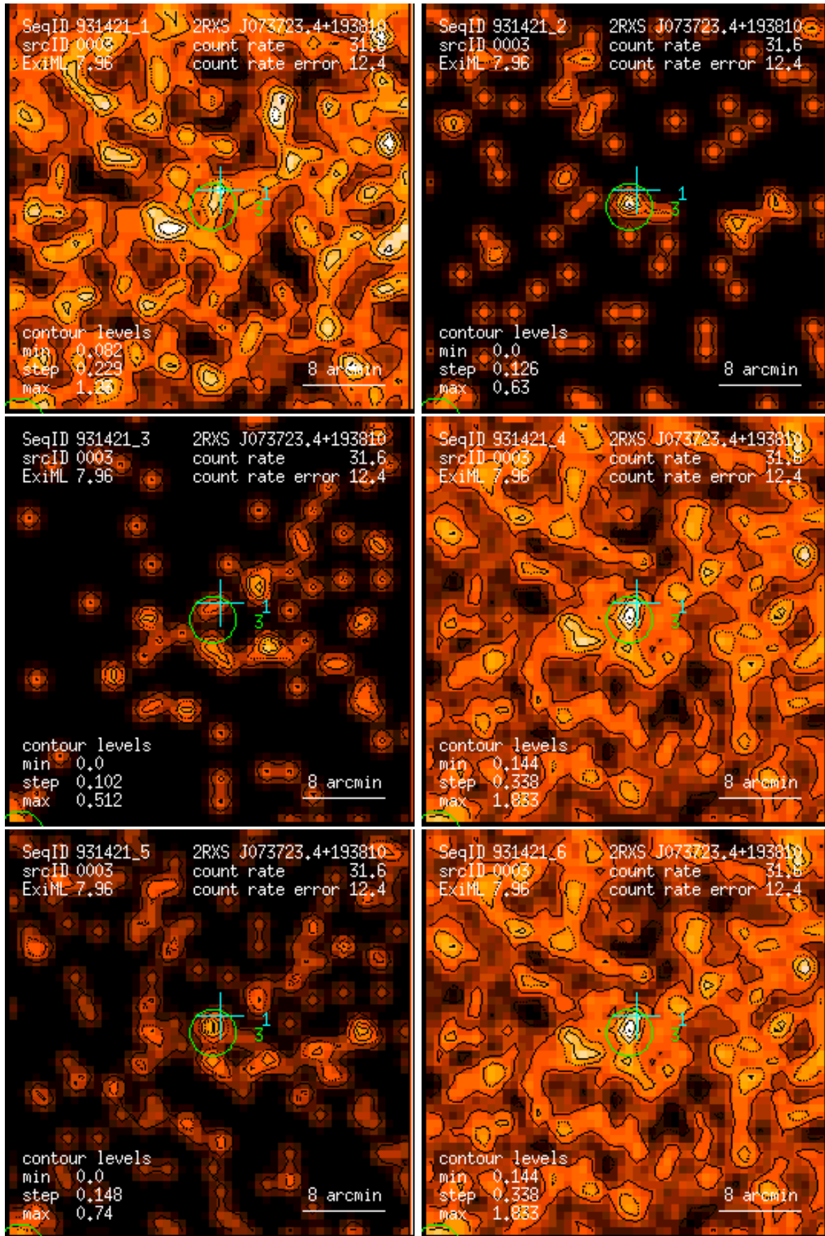
Figure 3: RASS 931421: detection 0003: band rate images, Gaussian filter: (1) PSPC channels 11 – 41, (2) 52 – 90, (3) 91 – 201, (4) 11 – 235, (5) 52 – 201, (6) 11 – 201. Broad band rates in counts/ks. Band rate contour levels in counts/ks/arcmin 2 .
