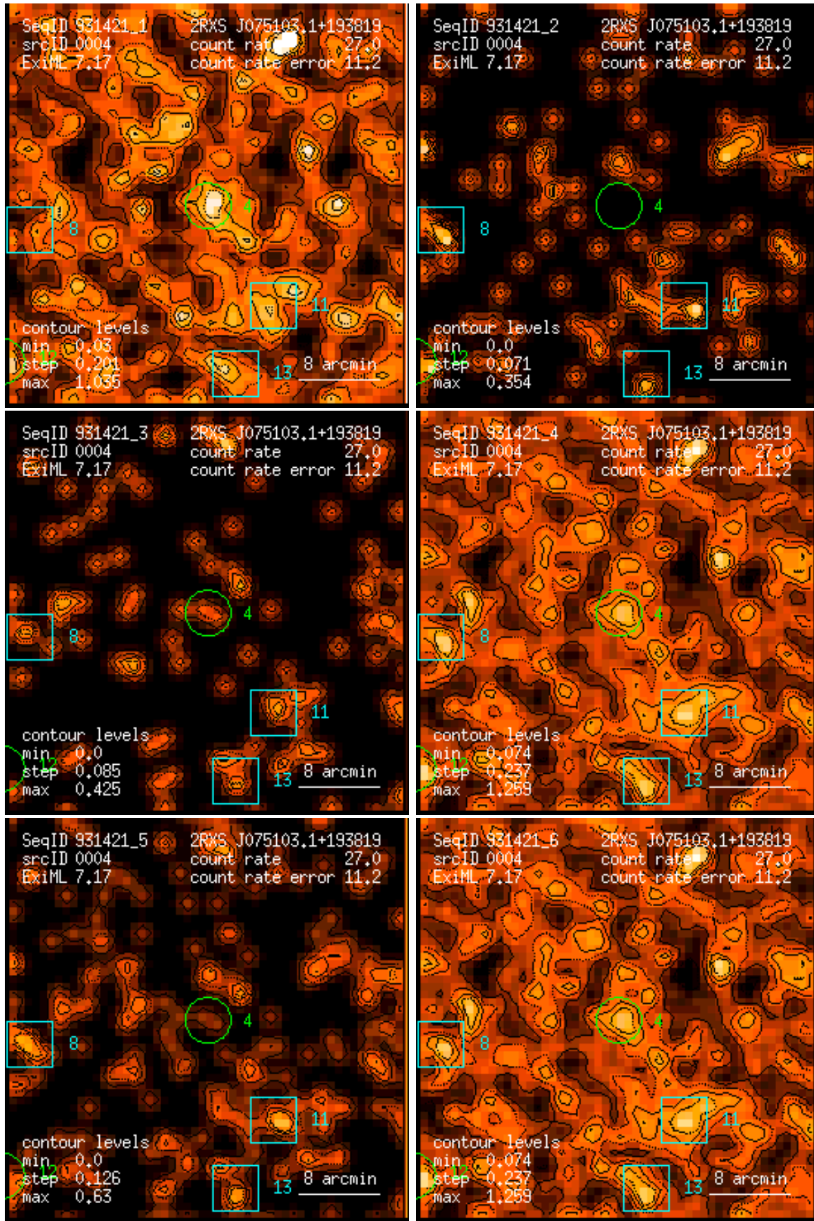
Figure 4: RASS 931421: detection 0004: band rate images, Gaussian filter: (1) PSPC channels 11 – 41, (2) 52 – 90, (3) 91 – 201, (4) 11 – 235, (5) 52 – 201, (6) 11 – 201. Broad band rates in counts/ks. Band rate contour levels in counts/ks/arcmin 2 .
