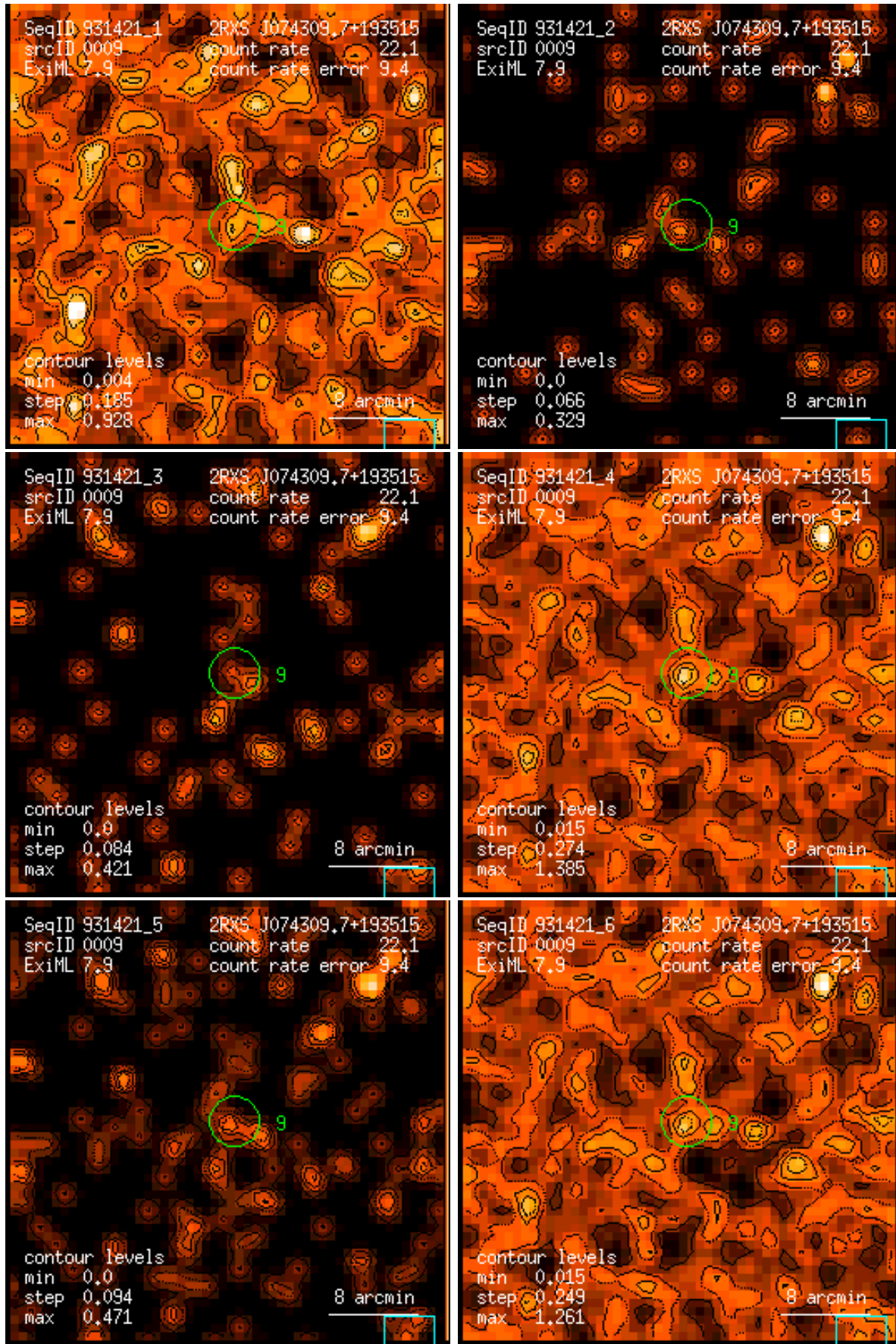
Figure 9: RASS 931421: detection 0009: band rate images, Gaussian filter: (1) PSPC channels 11 – 41, (2) 52 – 90, (3) 91 – 201, (4) 11 – 235, (5) 52 – 201, (6) 11 – 201. Broad band rates in counts/ks. Band rate contour levels in counts/ks/arcmin 2 .
