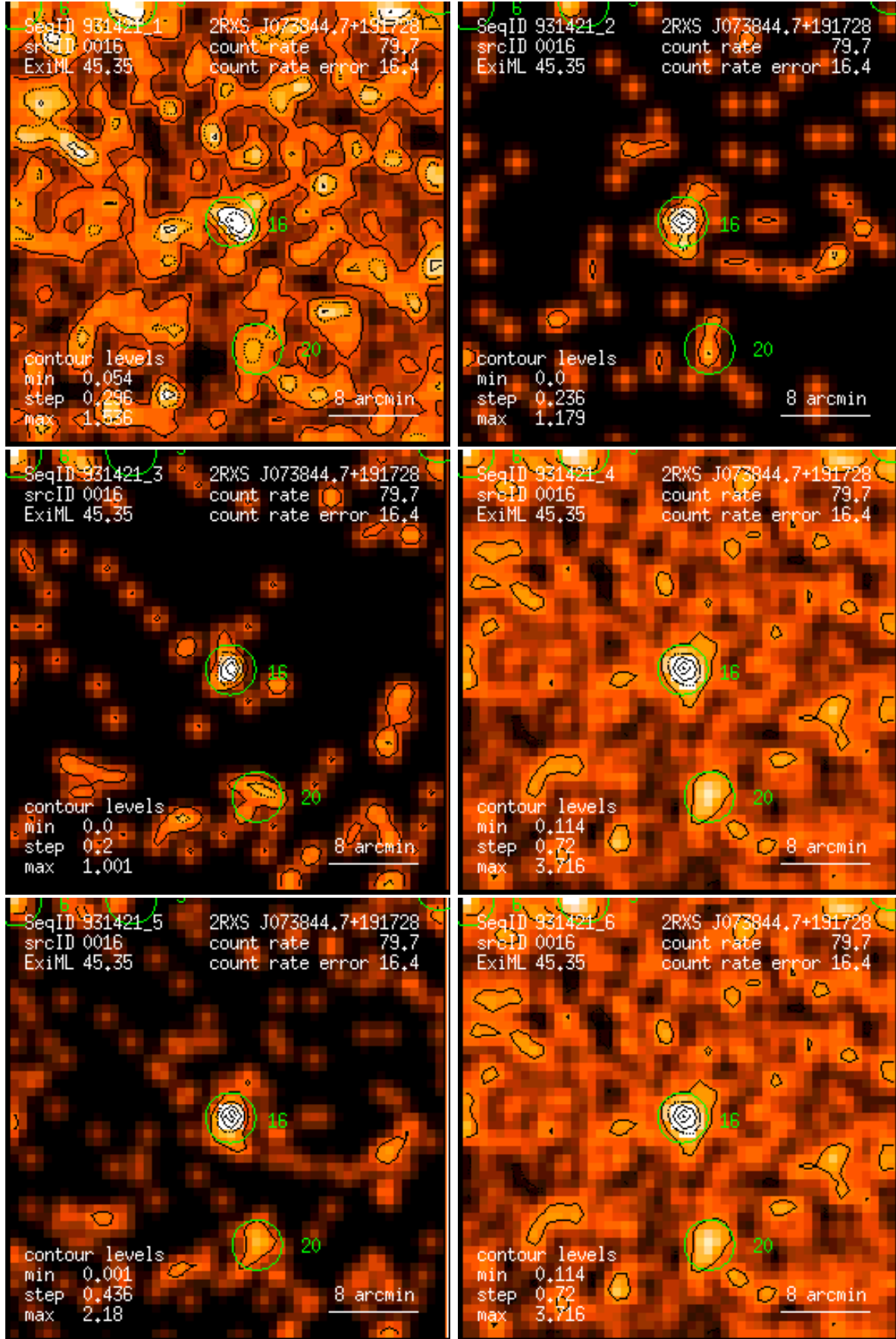
Figure 16: RASS 931421: detection 0016: band rate images, Gaussian filter: (1) PSPC channels 11 – 41, (2) 52 – 90, (3) 91 – 201, (4) 11 – 235, (5) 52 – 201, (6) 11 – 201. Broad band rates in counts/ks. Band rate contour levels in counts/ks/arcmin 2 .
