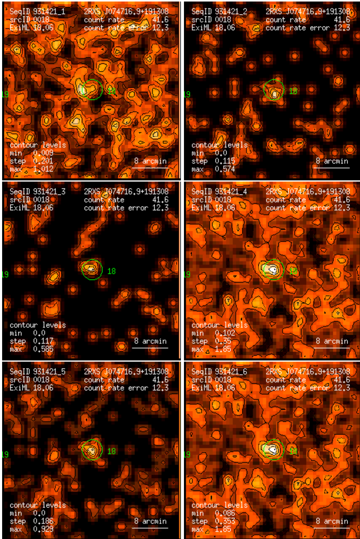
Figure 18: RASS 931421: detection 0018: band rate images, Gaussian filter: (1) PSPC channels 11 – 41, (2) 52 – 90, (3) 91 – 201, (4) 11 – 235, (5) 52 – 201, (6) 11 – 201. Broad band rates in counts/ks. Band rate contour levels in counts/ks/arcmin 2 .
