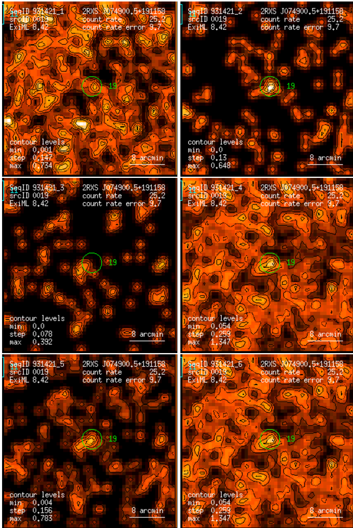
Figure 19: RASS 931421: detection 0019: band rate images, Gaussian filter: (1) PSPC channels 11 – 41, (2) 52 – 90, (3) 91 – 201, (4) 11 – 235, (5) 52 – 201, (6) 11 – 201. Broad band rates in counts/ks. Band rate contour levels in counts/ks/arcmin 2 .
