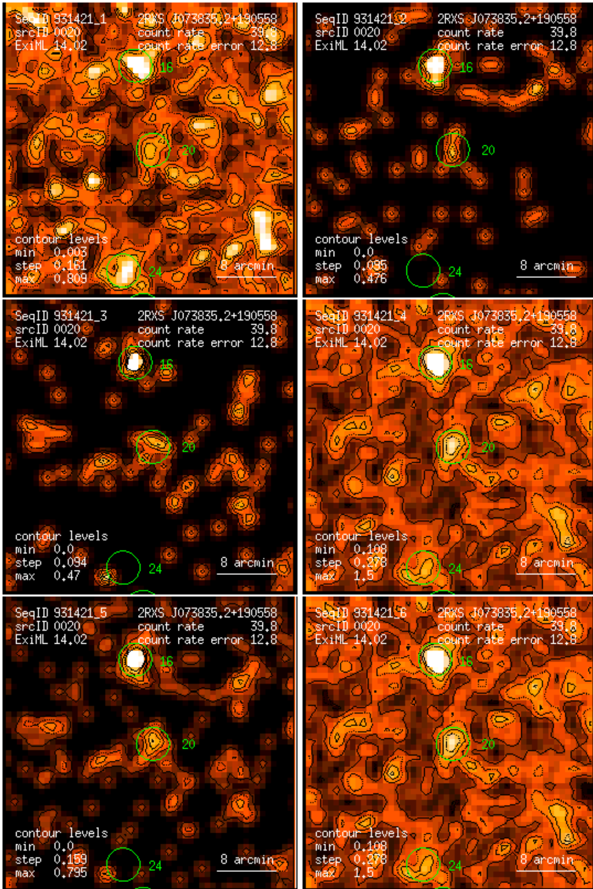
Figure 20: RASS 931421: detection 0020: band rate images, Gaussian filter: (1) PSPC channels 11 – 41, (2) 52 – 90, (3) 91 – 201, (4) 11 – 235, (5) 52 – 201, (6) 11 – 201. Broad band rates in counts/ks. Band rate contour levels in counts/ks/arcmin 2 .
