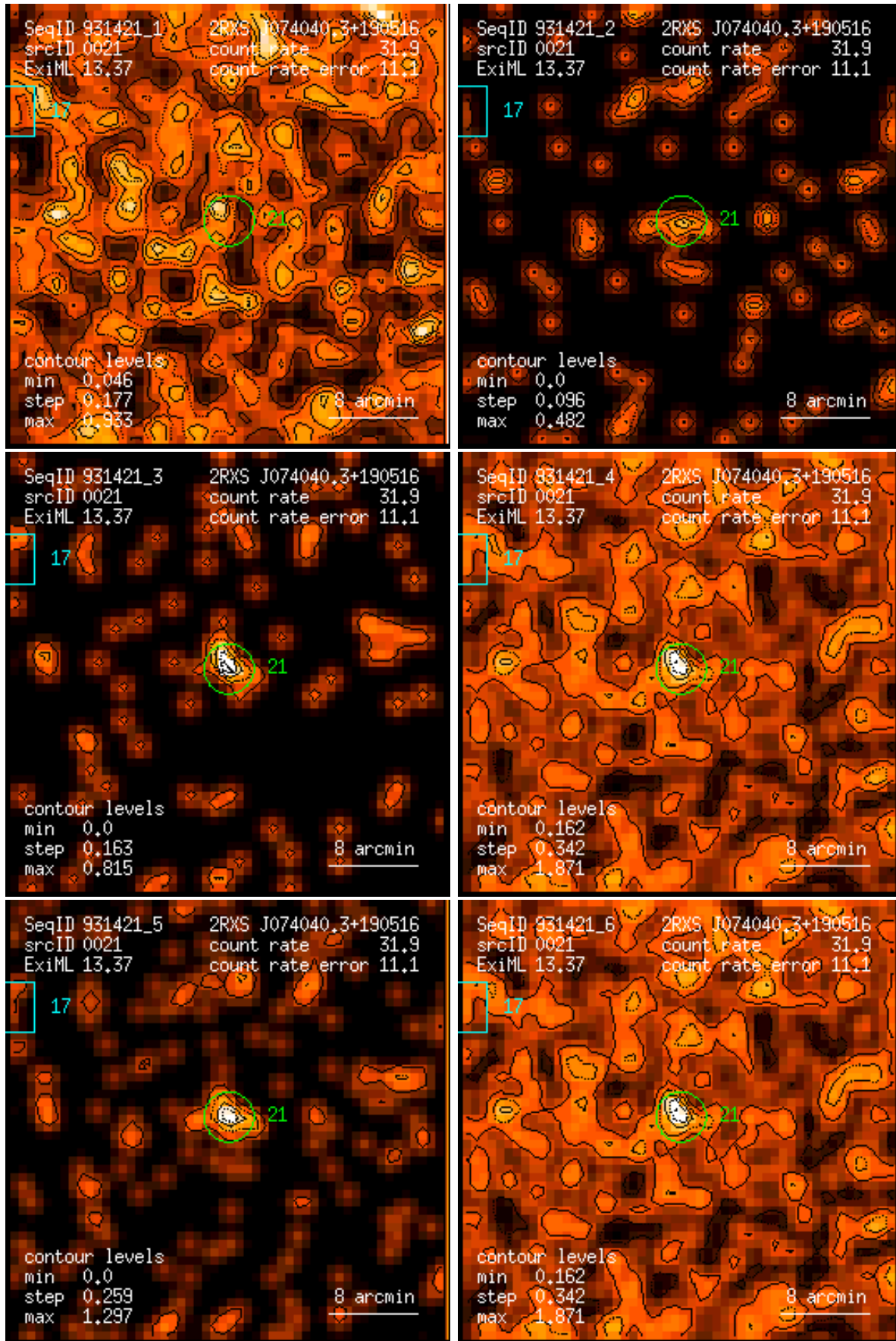
Figure 21: RASS 931421: detection 0021: band rate images, Gaussian filter: (1) PSPC channels 11 – 41, (2) 52 – 90, (3) 91 – 201, (4) 11 – 235, (5) 52 – 201, (6) 11 – 201. Broad band rates in counts/ks. Band rate contour levels in counts/ks/arcmin 2 .
