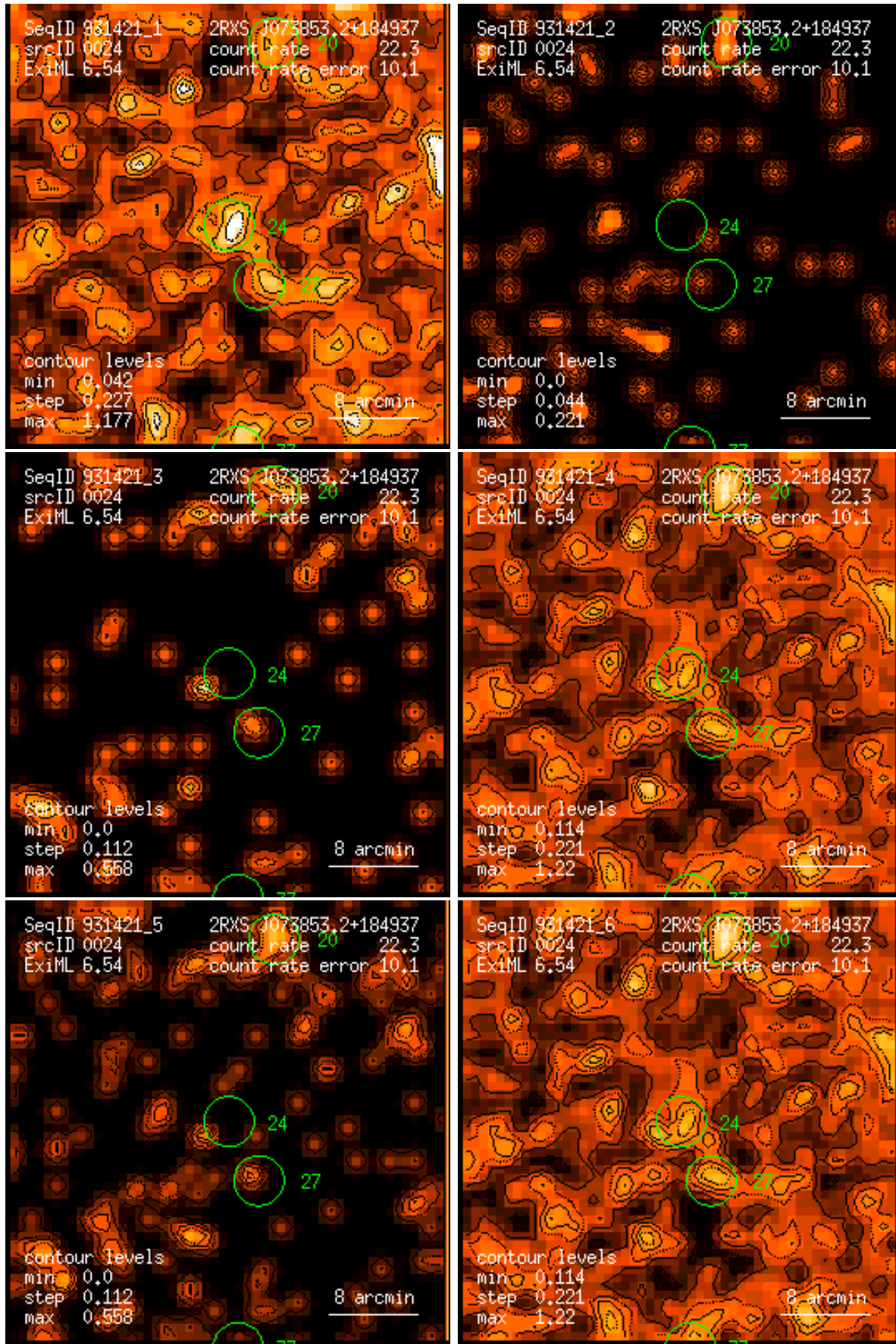
Figure 24: RASS 931421: detection 0024: band rate images, Gaussian filter: (1) PSPC channels 11 – 41, (2) 52 – 90, (3) 91 – 201, (4) 11 – 235, (5) 52 – 201, (6) 11 – 201. Broad band rates in counts/ks. Band rate contour levels in counts/ks/arcmin 2 .
