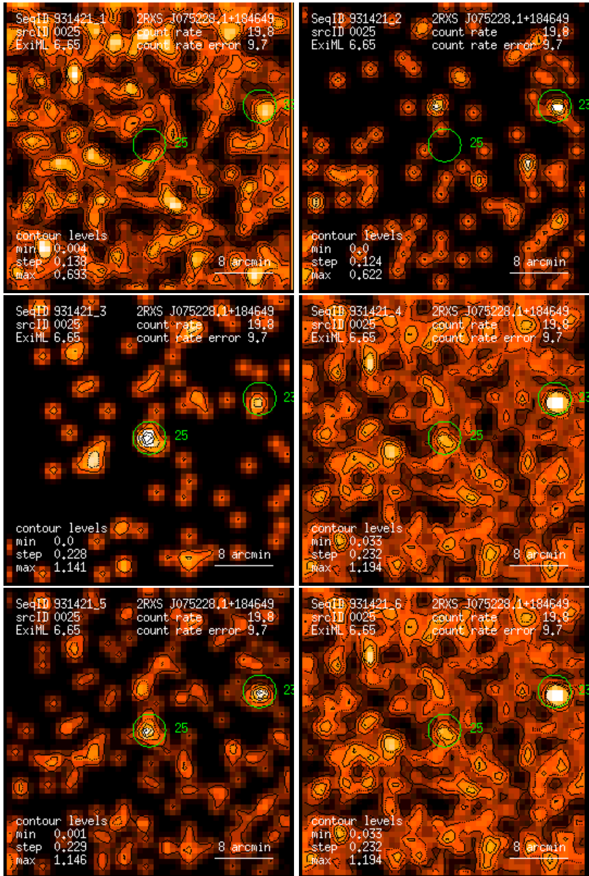
Figure 25: RASS 931421: detection 0025: band rate images, Gaussian filter: (1) PSPC channels 11 – 41, (2) 52 – 90, (3) 91 – 201, (4) 11 – 235, (5) 52 – 201, (6) 11 – 201. Broad band rates in counts/ks. Band rate contour levels in counts/ks/arcmin 2 .
