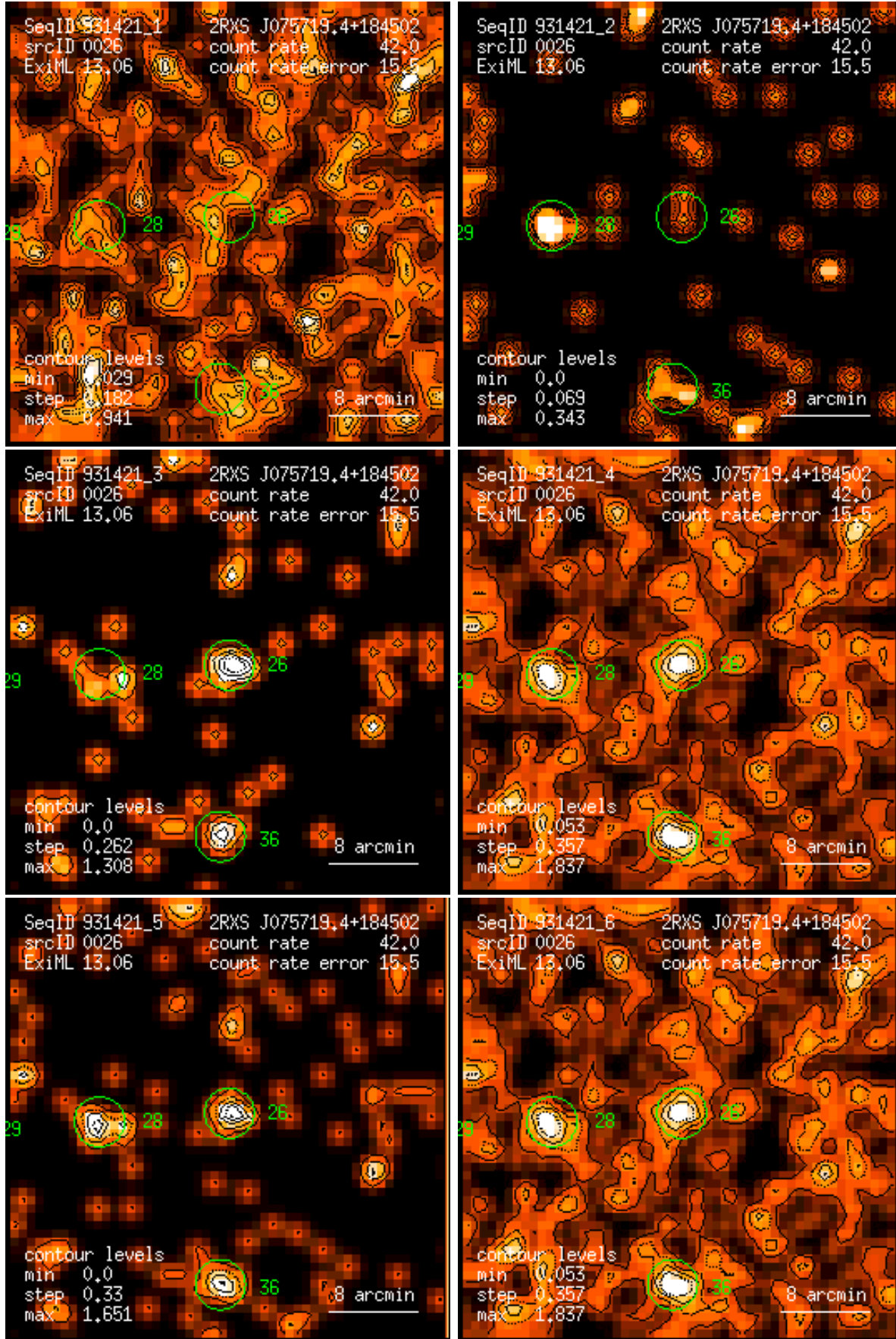
Figure 26: RASS 931421: detection 0026: band rate images, Gaussian filter: (1) PSPC channels 11 – 41, (2) 52 – 90, (3) 91 – 201, (4) 11 – 235, (5) 52 – 201, (6) 11 – 201. Broad band rates in counts/ks. Band rate contour levels in counts/ks/arcmin 2 .
