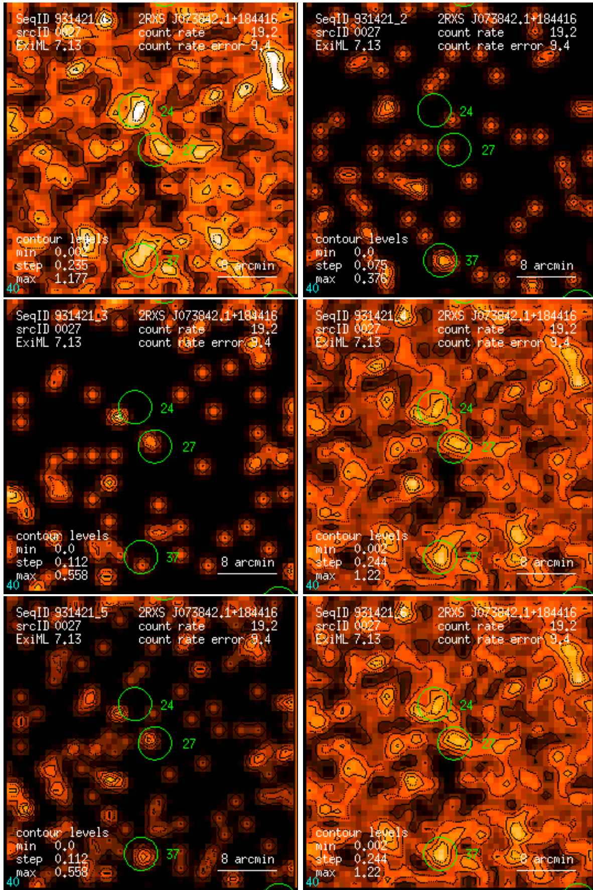
Figure 27: RASS 931421: detection 0027: band rate images, Gaussian filter: (1) PSPC channels 11 – 41, (2) 52 – 90, (3) 91 – 201, (4) 11 – 235, (5) 52 – 201, (6) 11 – 201. Broad band rates in counts/ks. Band rate contour levels in counts/ks/arcmin 2 .
