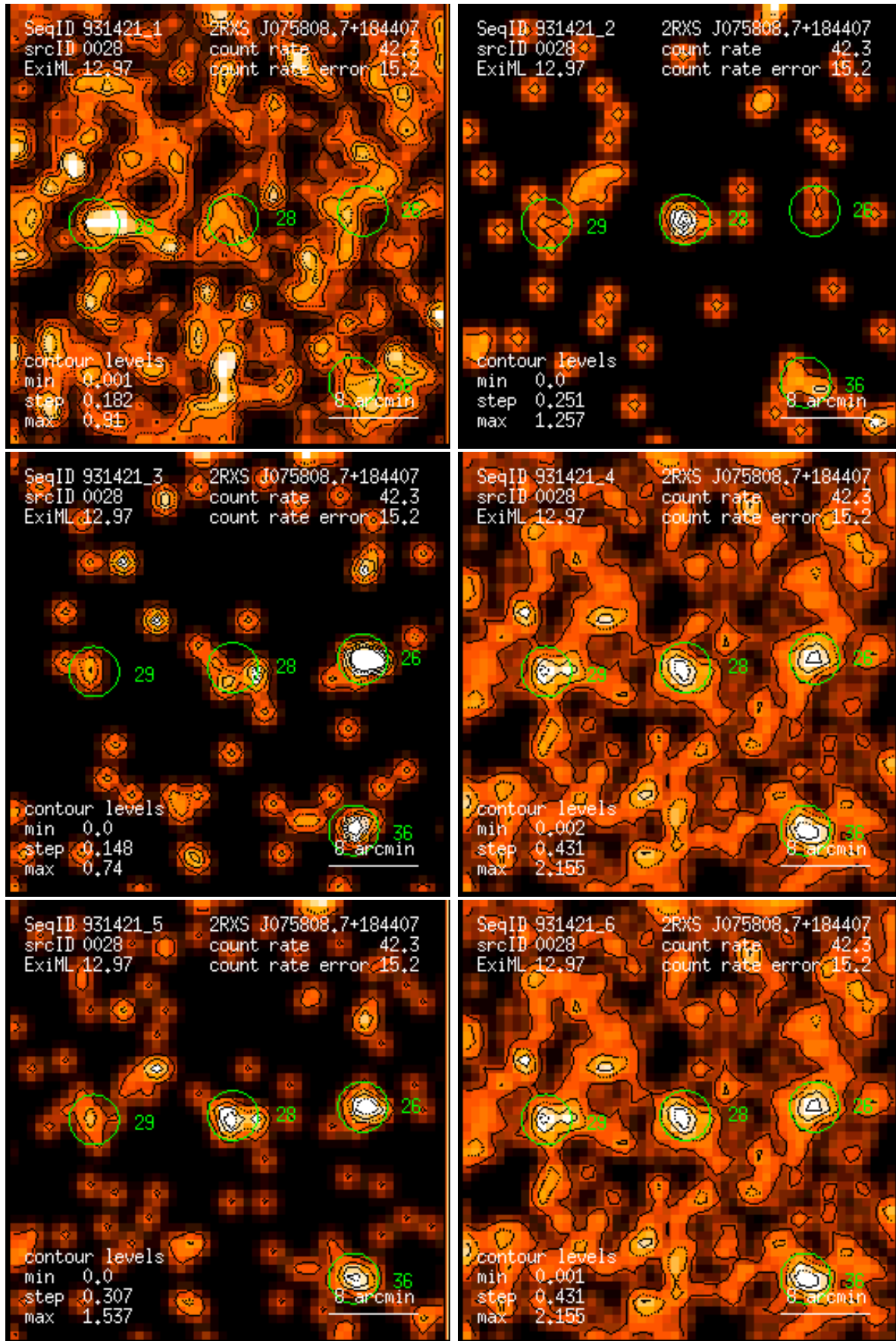
Figure 28: RASS 931421: detection 0028: band rate images, Gaussian filter: (1) PSPC channels 11 – 41, (2) 52 – 90, (3) 91 – 201, (4) 11 – 235, (5) 52 – 201, (6) 11 – 201. Broad band rates in counts/ks. Band rate contour levels in counts/ks/arcmin 2 .
