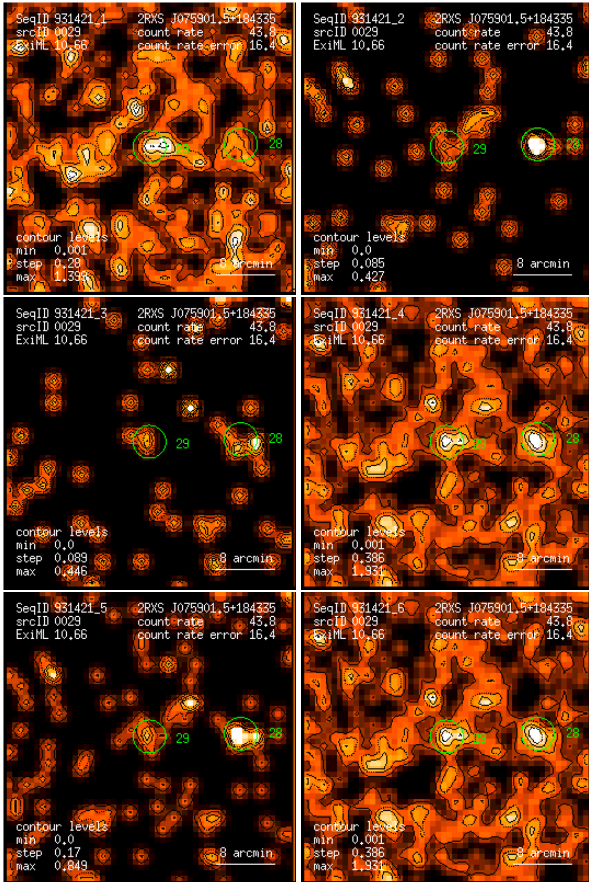
Figure 29: RASS 931421: detection 0029: band rate images, Gaussian filter: (1) PSPC channels 11 – 41, (2) 52 – 90, (3) 91 – 201, (4) 11 – 235, (5) 52 – 201, (6) 11 – 201. Broad band rates in counts/ks. Band rate contour levels in counts/ks/arcmin 2 .
