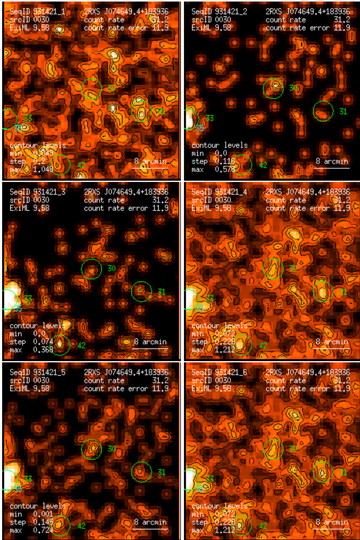
Figure 30: RASS 931421: detection 0030: band rate images, Gaussian filter: (1) PSPC channels 11 – 41, (2) 52 – 90, (3) 91 – 201, (4) 11 – 235, (5) 52 – 201, (6) 11 – 201. Broad band rates in counts/ks. Band rate contour levels in counts/ks/arcmin 2 .
