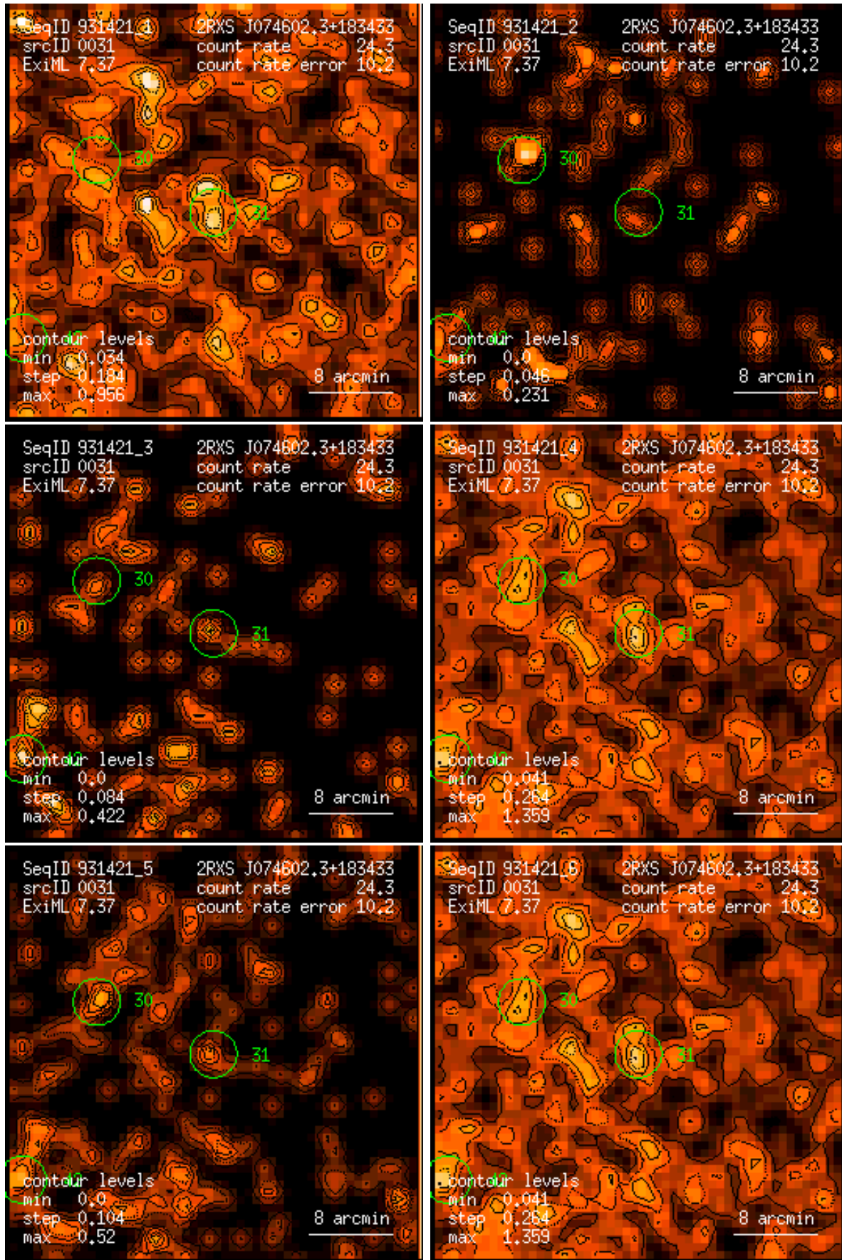
Figure 31: RASS 931421: detection 0031: band rate images, Gaussian filter: (1) PSPC channels 11 – 41, (2) 52 – 90, (3) 91 – 201, (4) 11 – 235, (5) 52 – 201, (6) 11 – 201. Broad band rates in counts/ks. Band rate contour levels in counts/ks/arcmin 2 .
