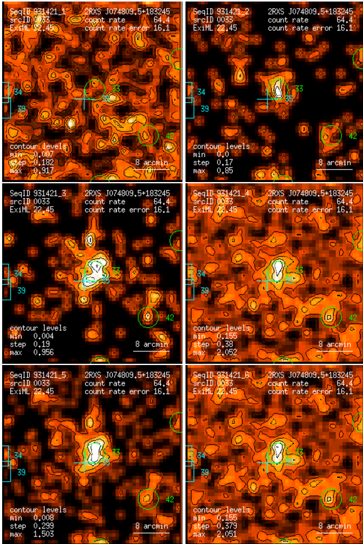
Figure 33: RASS 931421: detection 0033: band rate images, Gaussian filter: (1) PSPC channels 11 – 41, (2) 52 – 90, (3) 91 – 201, (4) 11 – 235, (5) 52 – 201, (6) 11 – 201. Broad band rates in counts/ks. Band rate contour levels in counts/ks/arcmin 2 .
