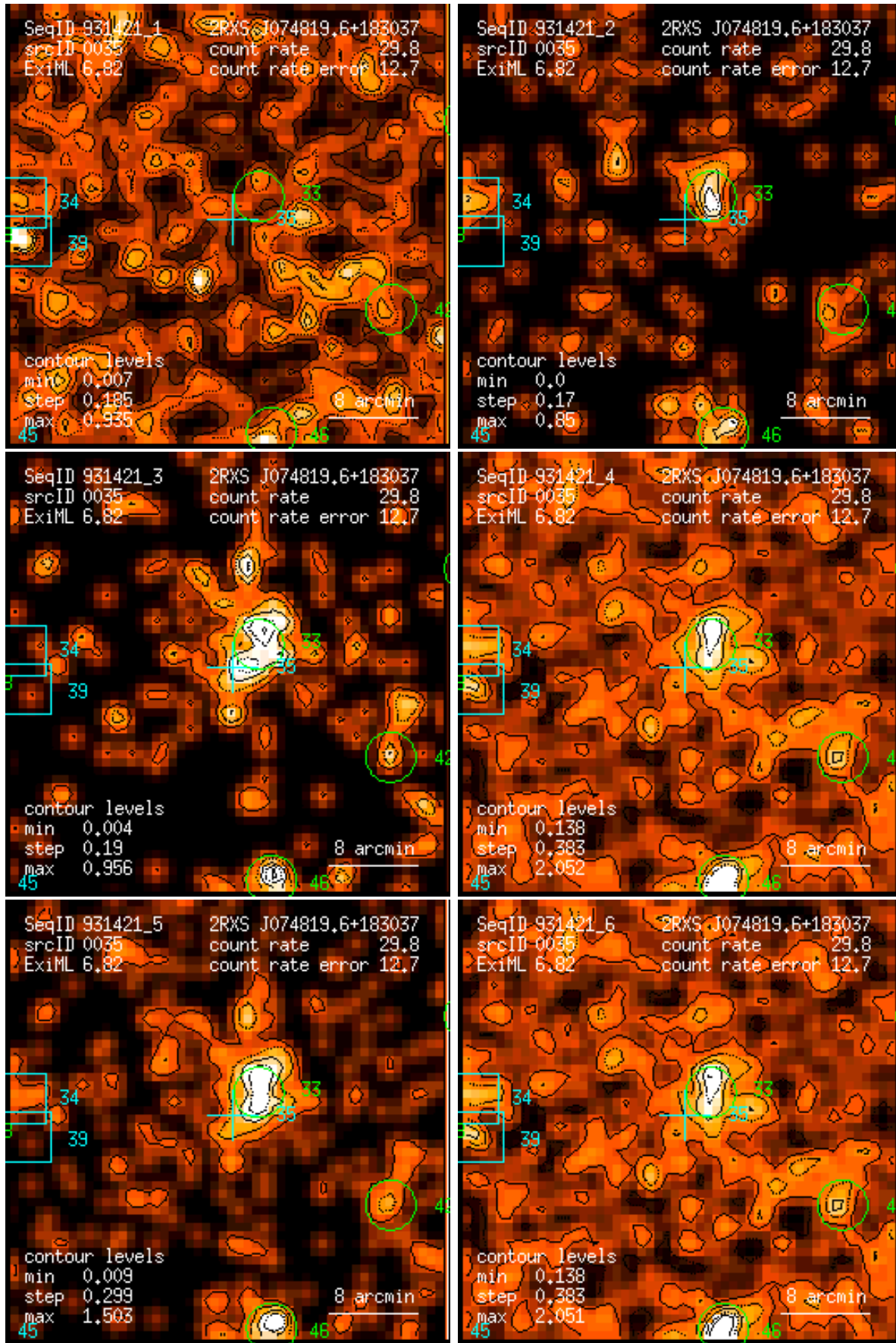
Figure 35: RASS 931421: detection 0035: band rate images, Gaussian filter: (1) PSPC channels 11 – 41, (2) 52 – 90, (3) 91 – 201, (4) 11 – 235, (5) 52 – 201, (6) 11 – 201. Broad band rates in counts/ks. Band rate contour levels in counts/ks/arcmin 2 .
