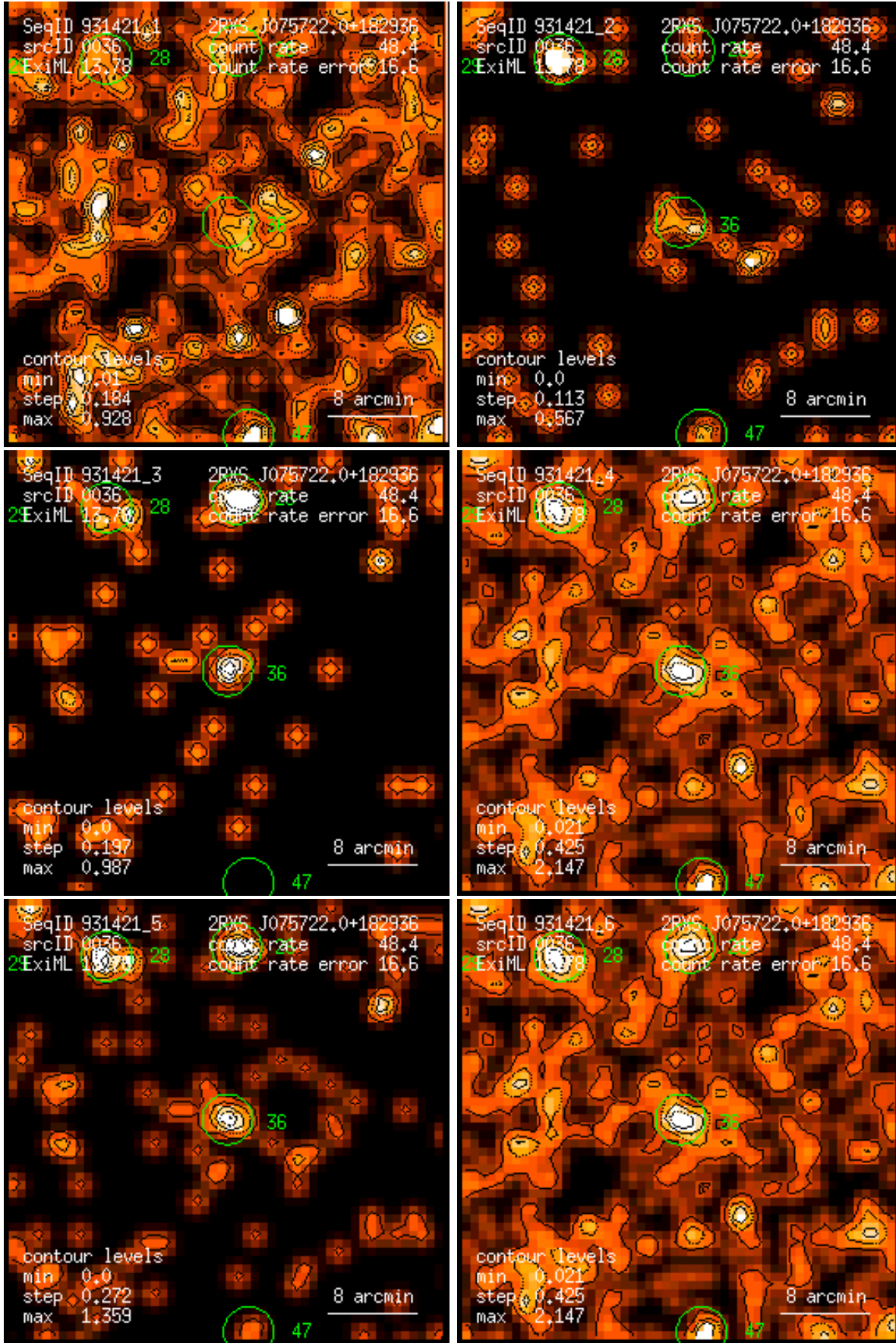
Figure 36: RASS 931421: detection 0036: band rate images, Gaussian filter: (1) PSPC channels 11 – 41, (2) 52 – 90, (3) 91 – 201, (4) 11 – 235, (5) 52 – 201, (6) 11 – 201. Broad band rates in counts/ks. Band rate contour levels in counts/ks/arcmin 2 .
