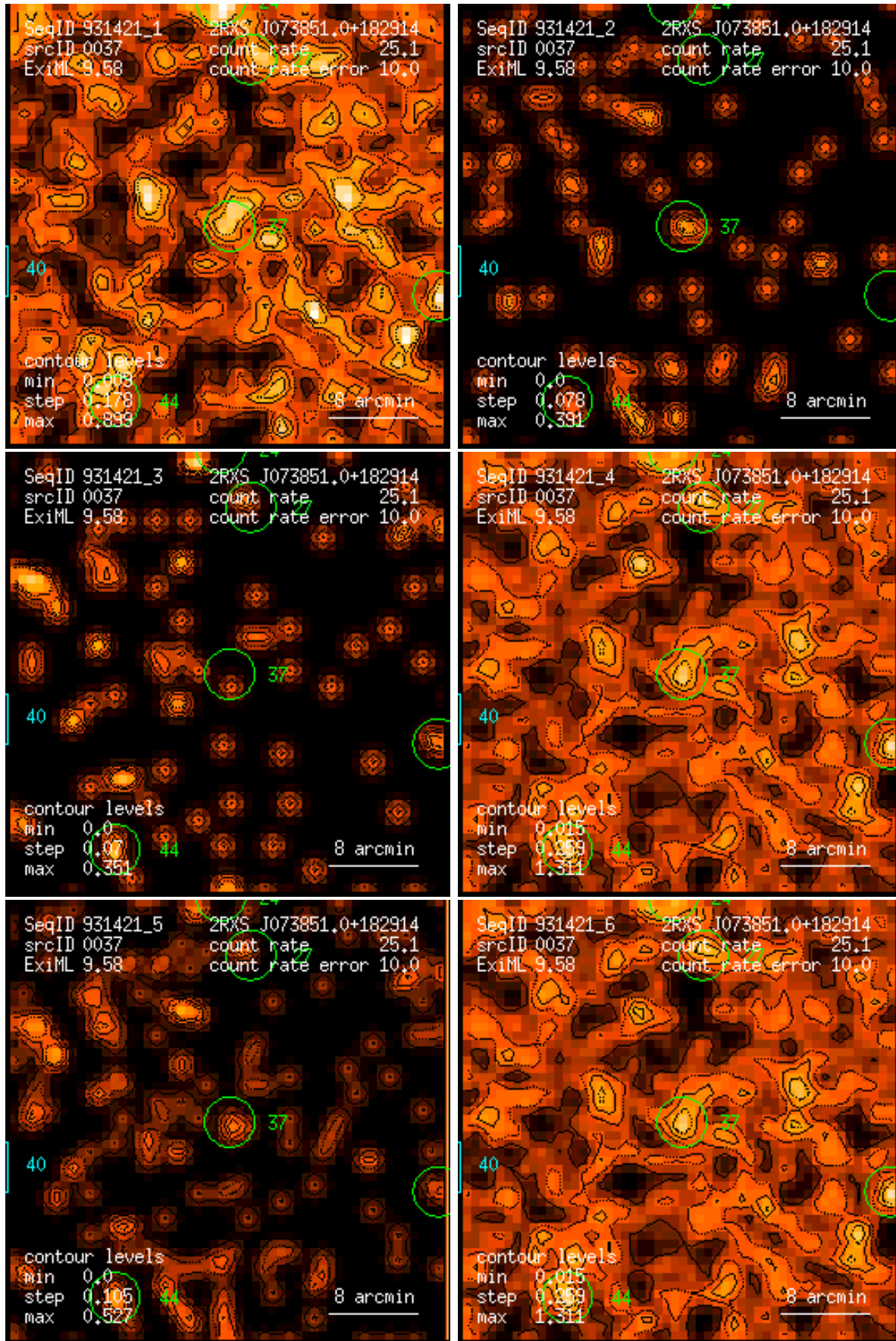
Figure 37: RASS 931421: detection 0037: band rate images, Gaussian filter: (1) PSPC channels 11 – 41, (2) 52 – 90, (3) 91 – 201, (4) 11 – 235, (5) 52 – 201, (6) 11 – 201. Broad band rates in counts/ks. Band rate contour levels in counts/ks/arcmin 2 .
