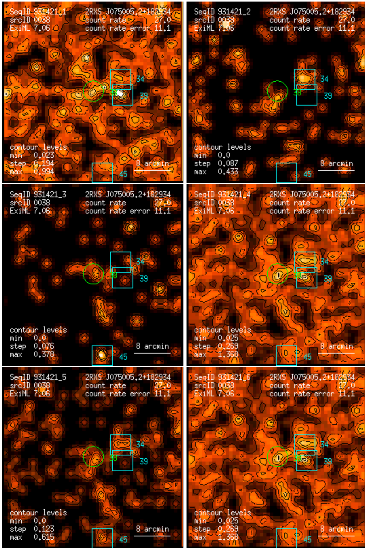
Figure 38: RASS 931421: detection 0038: band rate images, Gaussian filter: (1) PSPC channels 11 – 41, (2) 52 – 90, (3) 91 – 201, (4) 11 – 235, (5) 52 – 201, (6) 11 – 201. Broad band rates in counts/ks. Band rate contour levels in counts/ks/arcmin 2 .
